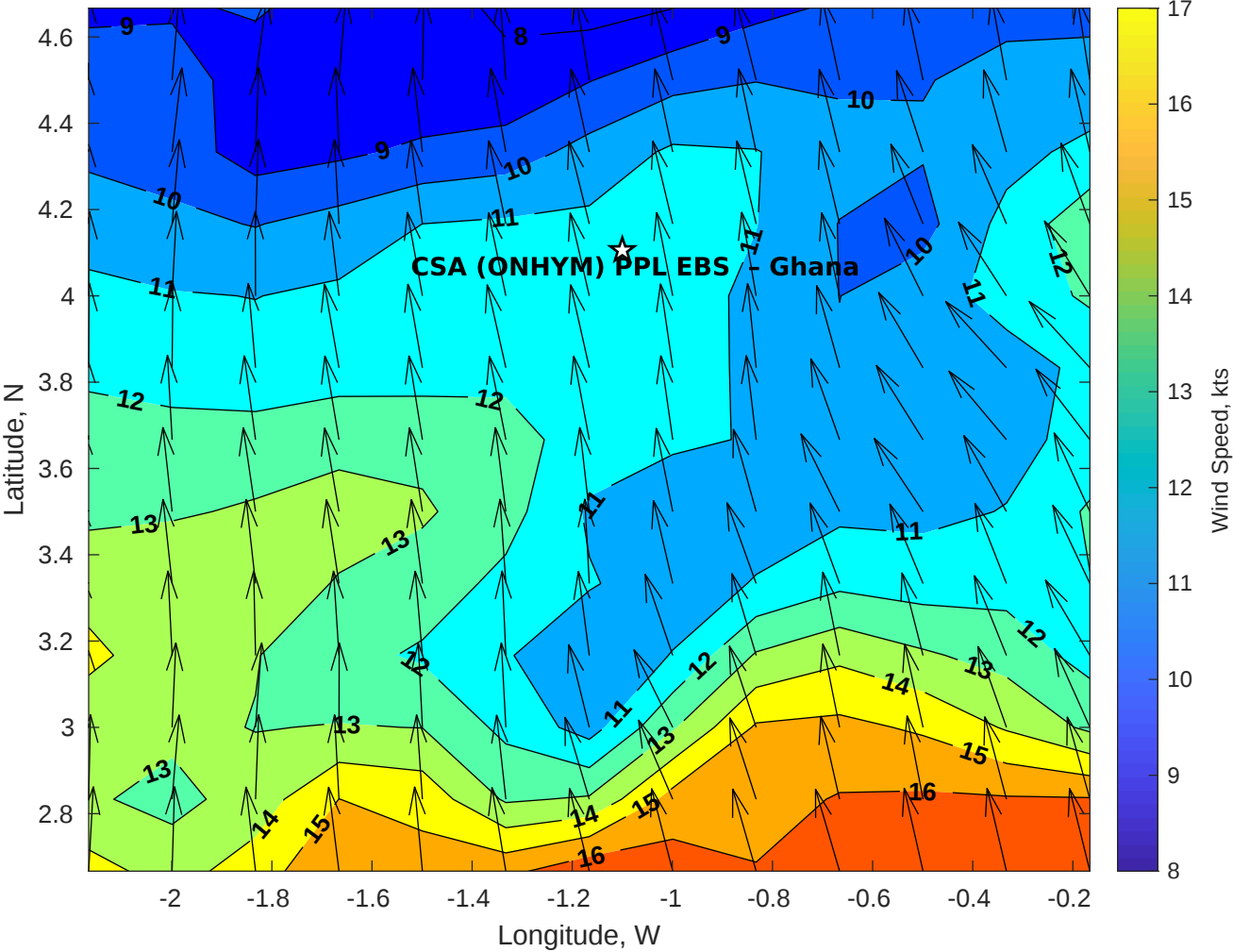
Winds (kts) for CSA (ONHYM) PPL EBS - Ghana at 21-May-2025 09:00:00
