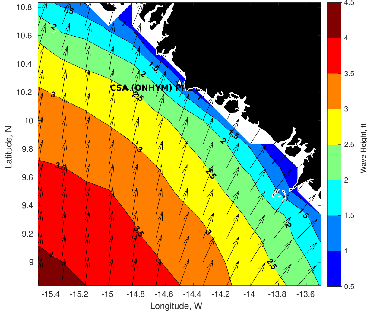
Wave Height (ft) for CSA (ONHYM) PPL EBS - Guinea at 21-May-2025 09:00:00
