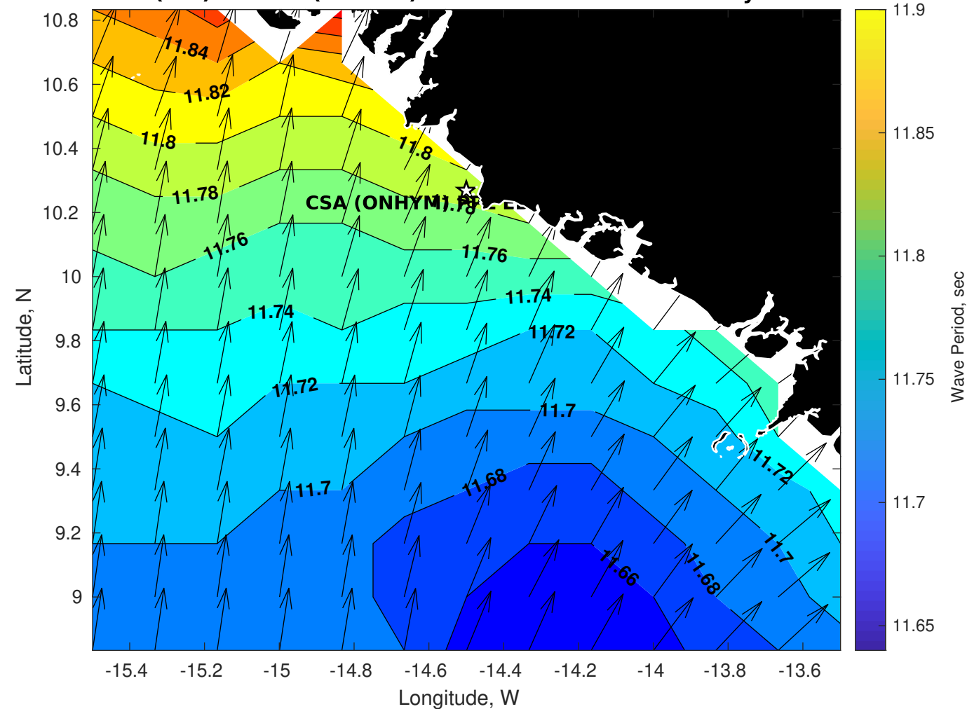
Wave Period (sec) for CSA (ONHYM) PPL EBS - Guinea at 21-May-2025 09:00:00
