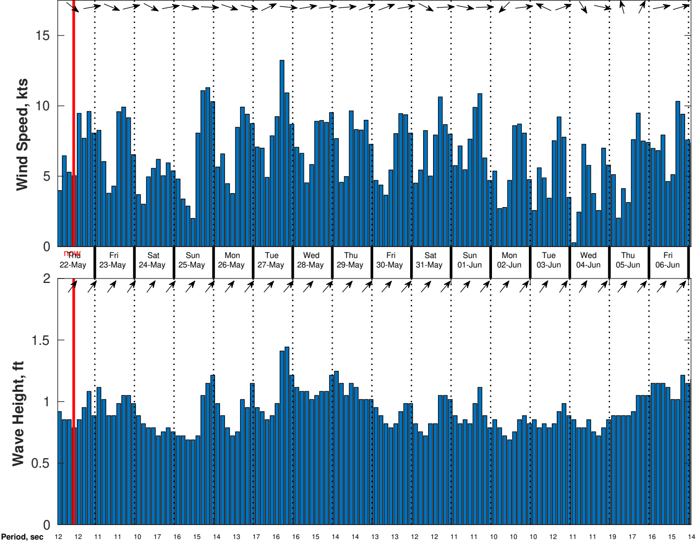
Wind & Wave Forecast for CSA (ONHYM) PPL EBS - Guinea from 21-May-2025 01:00:00 to 06-Jun-2025 01:00:00
