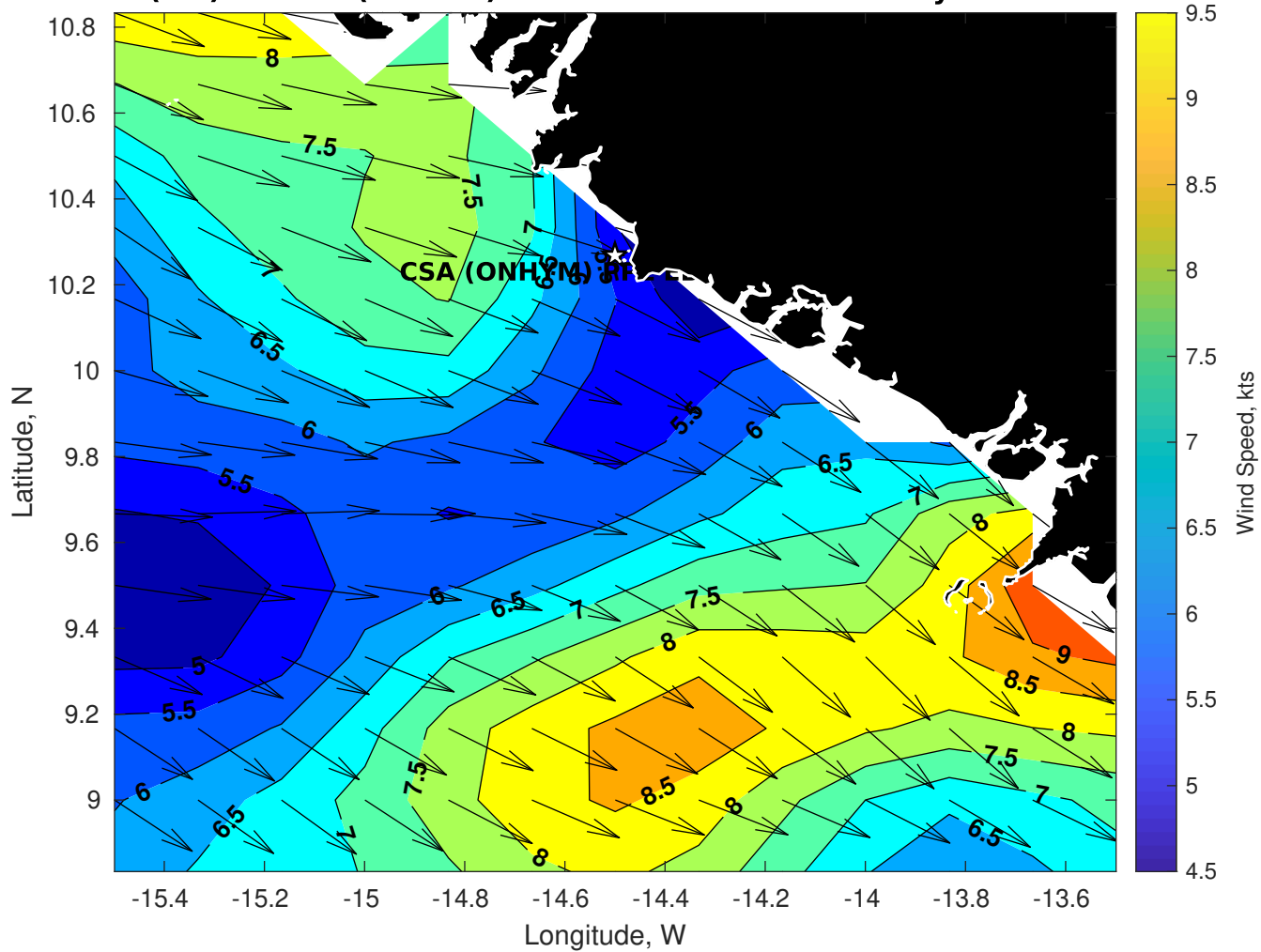
Winds (kts) for CSA (ONHYM) PPL EBS - Guinea at 21-May-2025 09:00:00
