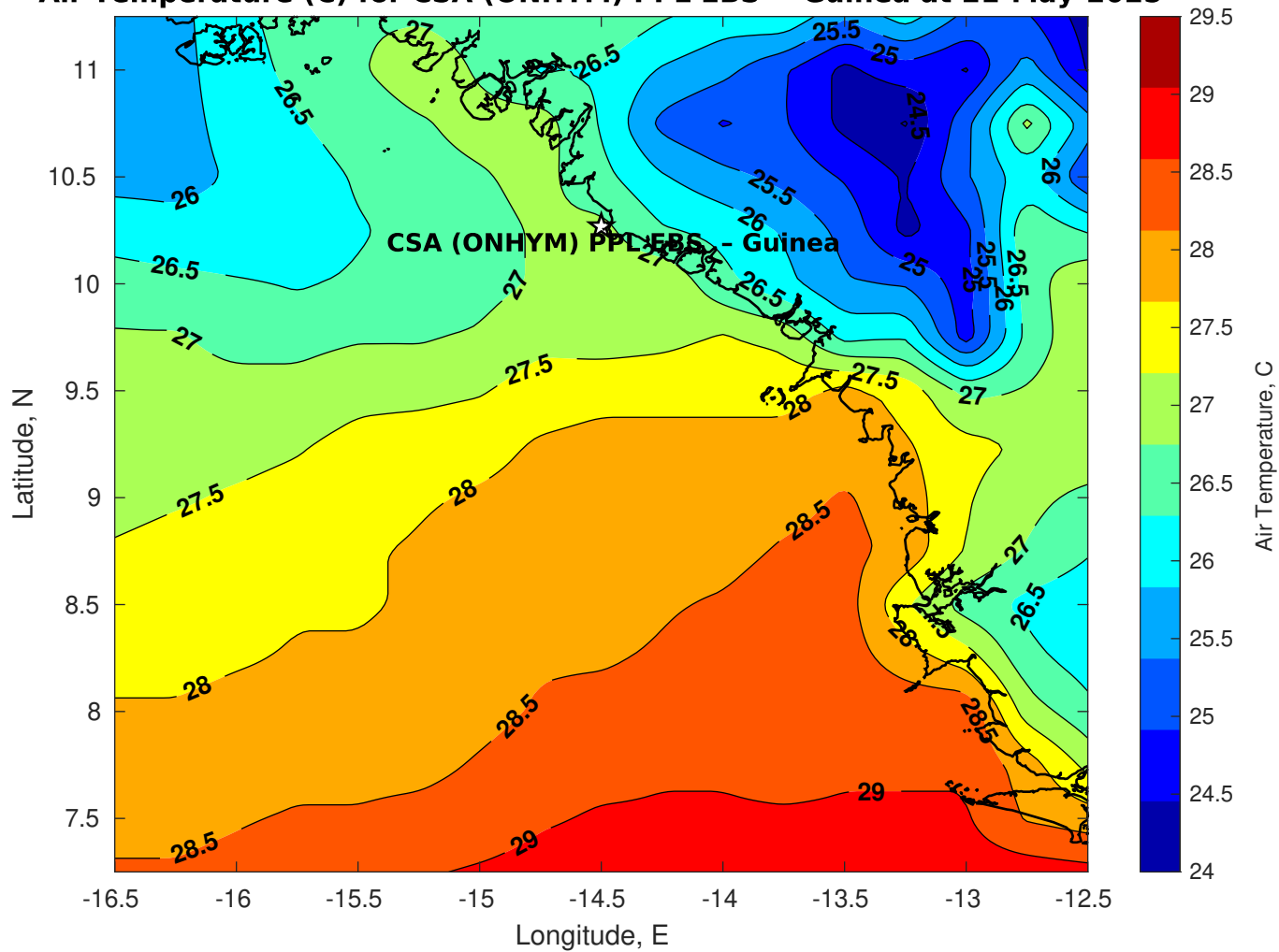
Air Temperature (C) for CSA (ONHYM) PPL EBS - Guinea at 21-May-2025
