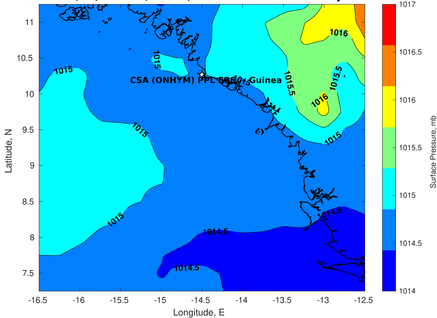
Surface Pressure (mb) for CSA (ONHYM) PPL EBS - Guinea at 23-May-2025 00:00:00
