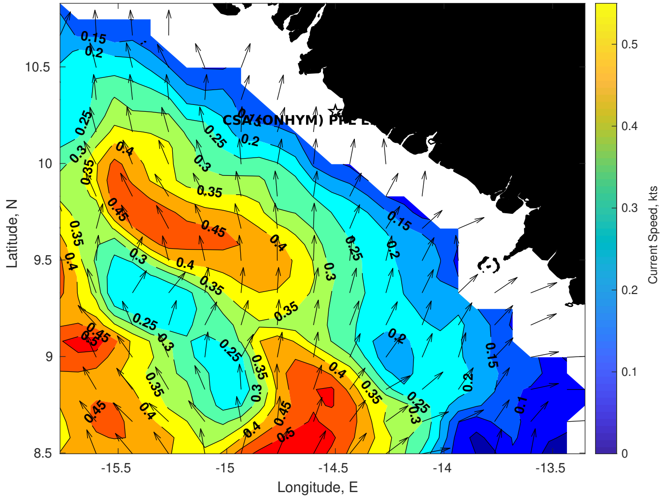
Surface Currents for CSA (ONHYM) PPL EBS - Guinea at 20-May-2025 00:00:00
