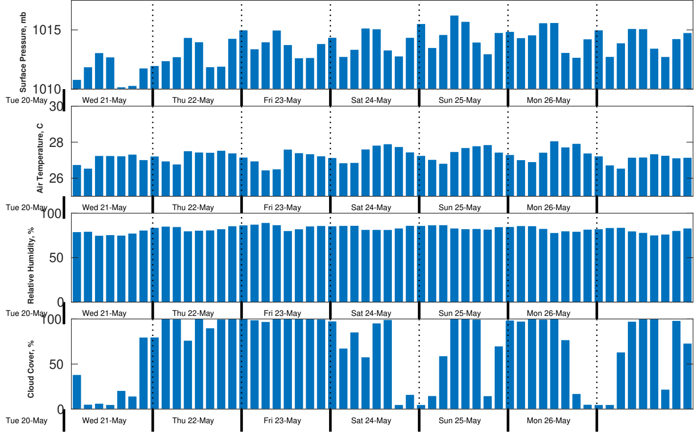
Met Forecast for CSA (ONHYM) PPL EBS - Guinea from 21-May-2025 00:00:00 to 28-May-2025 00:00:00
