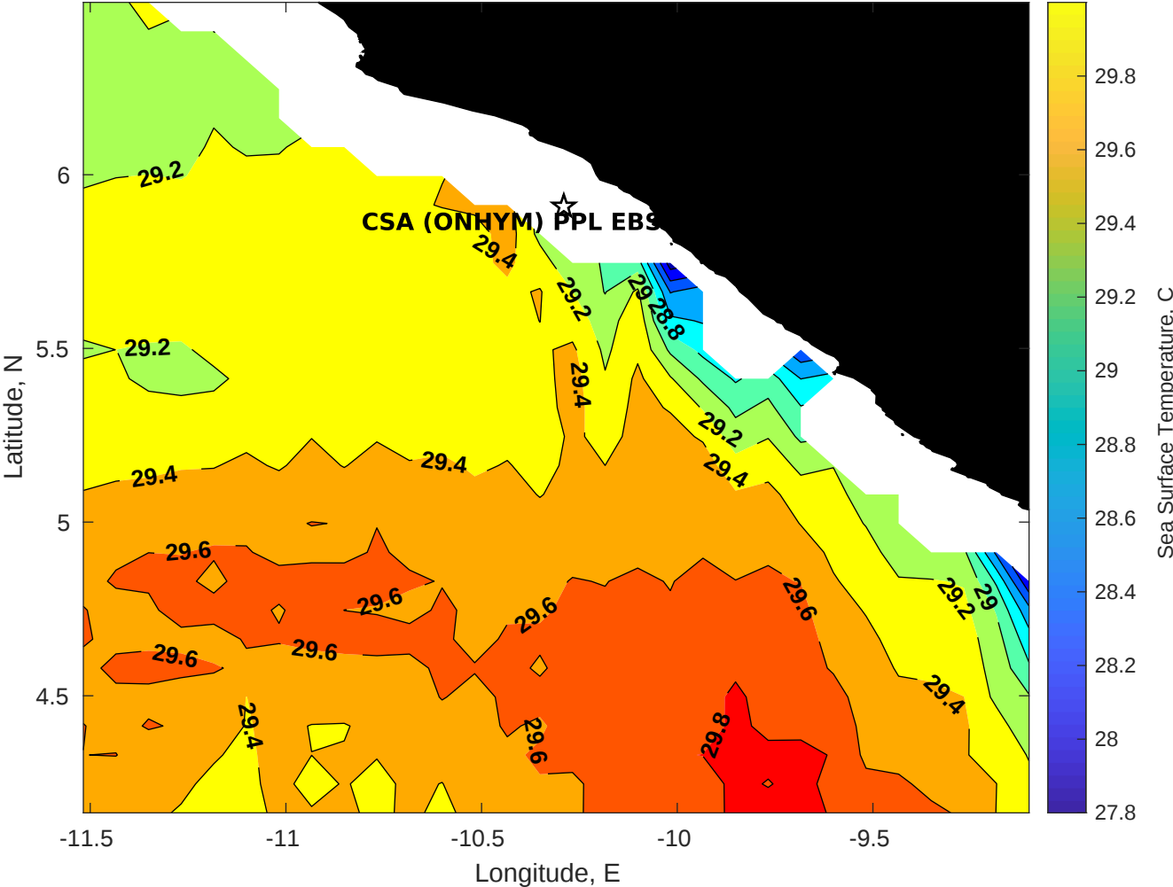
SST for CSA (ONHYM) PPL EBS - Liberia at 20-May-2025 00:00:00
