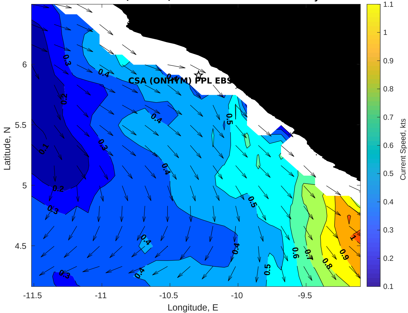
Surface Currents for CSA (ONHYM) PPL EBS - Liberia at 20-May-2025 00:00:00
