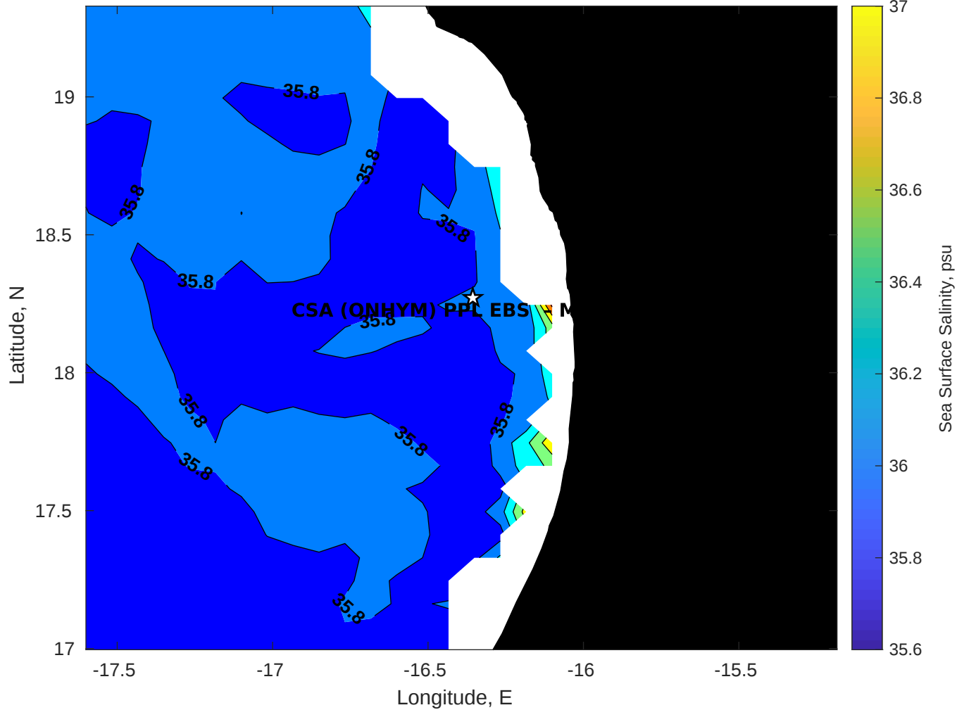
Surface Salinity for CSA (ONHYM) PPL EBS - Mauritania at 20-May-2025 00:00:00
