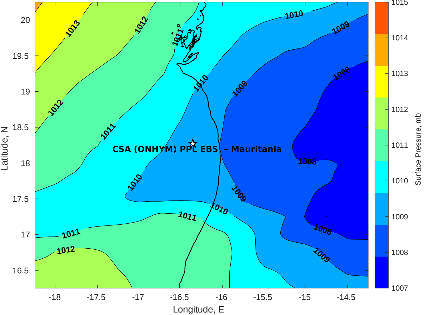
Surface Pressure (mb) for CSA (ONHYM) PPL EBS - Mauritania at 23-May-2025 00:00:00
