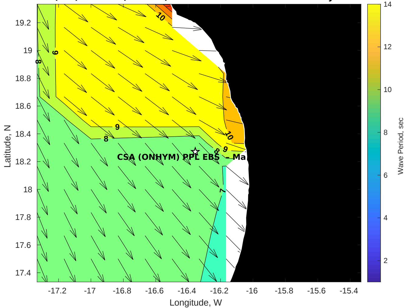
Wave Period (sec) for CSA (ONHYM) PPL EBS - Mauritania at 21-May-2025 09:00:00
