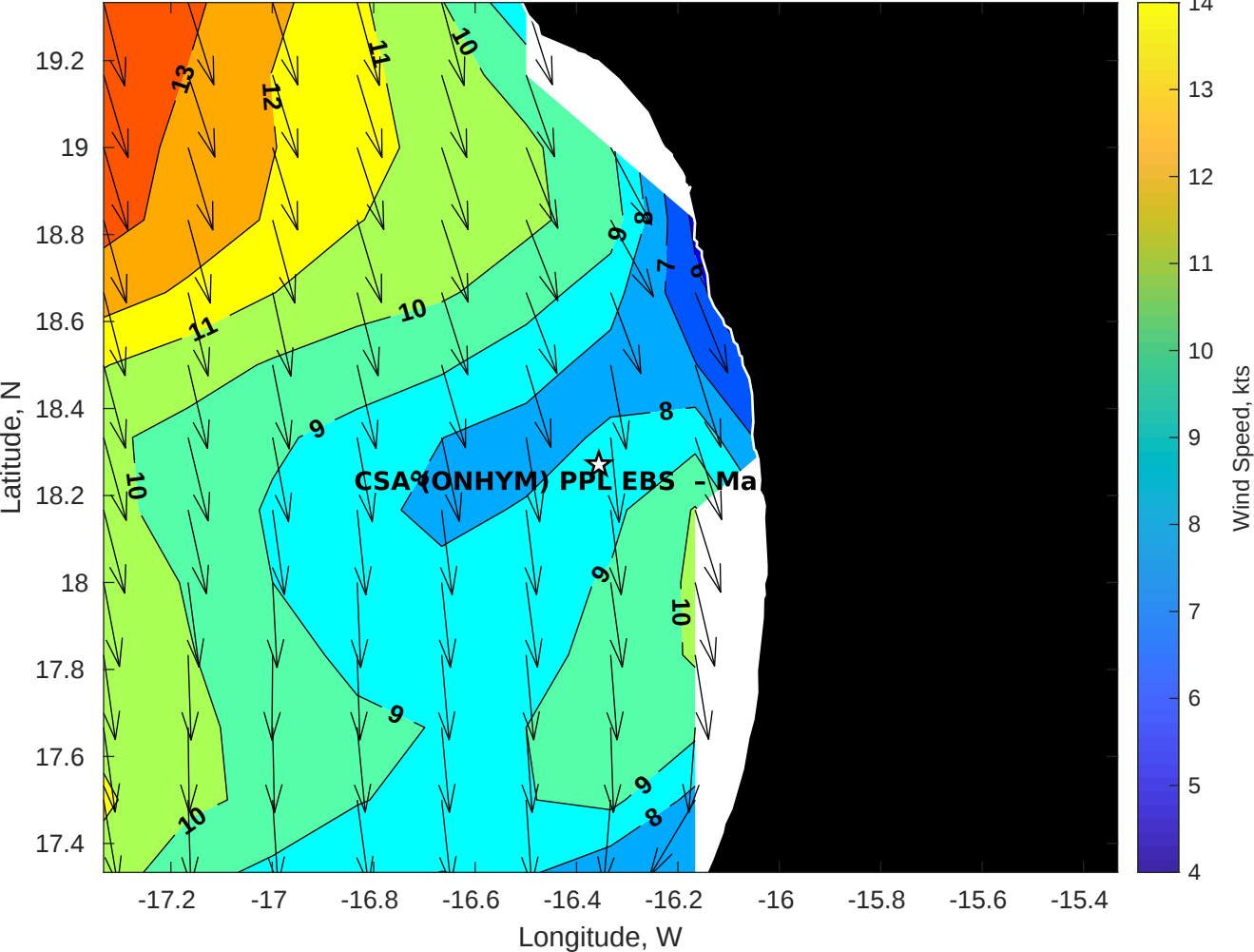
Winds (kts) for CSA (ONHYM) PPL EBS - Mauritania at 21-May-2025 09:00:00
