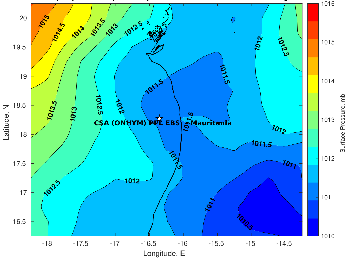
Surface Pressure (mb) for CSA (ONHYM) PPL EBS - Mauritania at 21-May-2025 00:00:00
