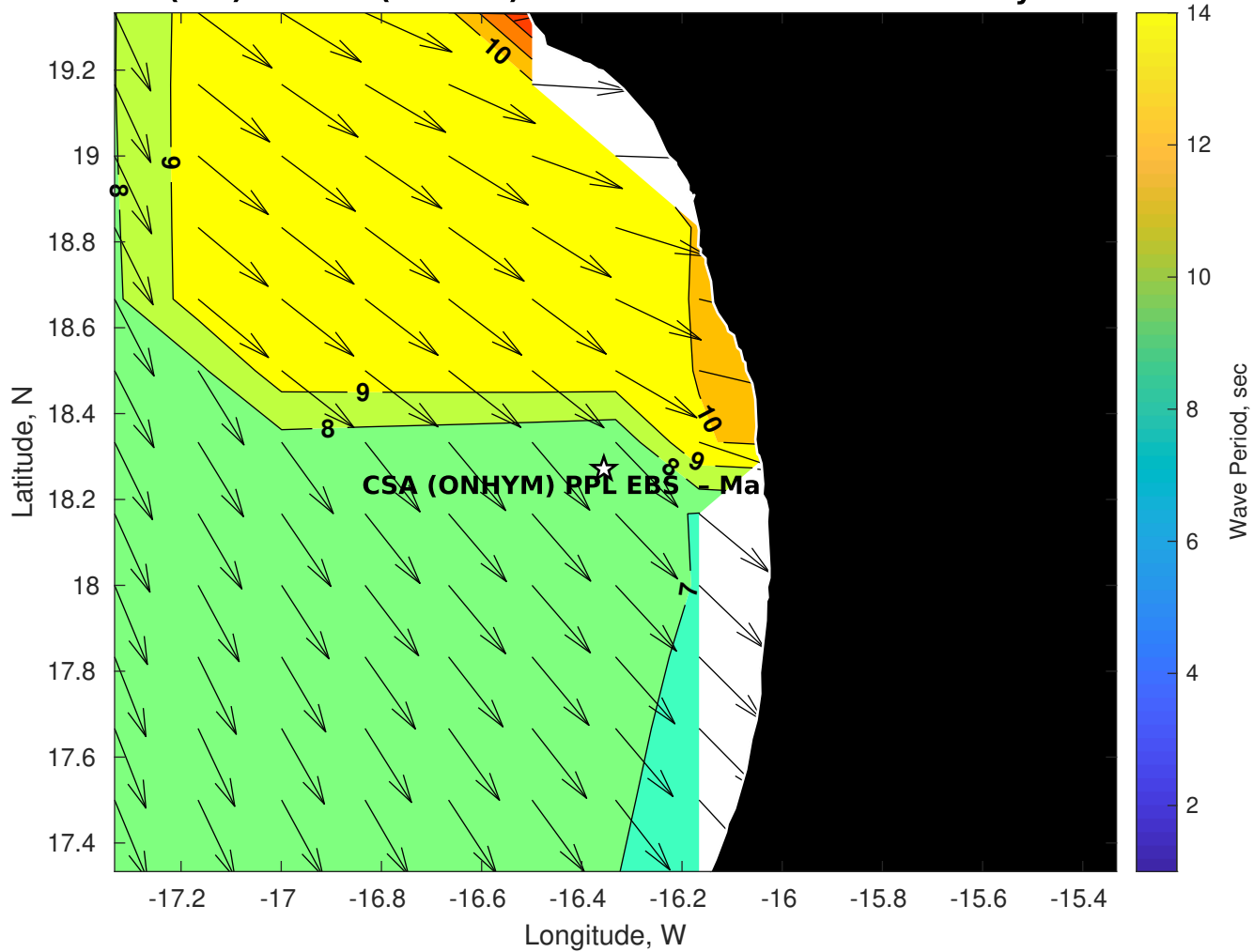
Wave Period (sec) for CSA (ONHYM) PPL EBS - Mauritania at 21-May-2025 09:00:00
