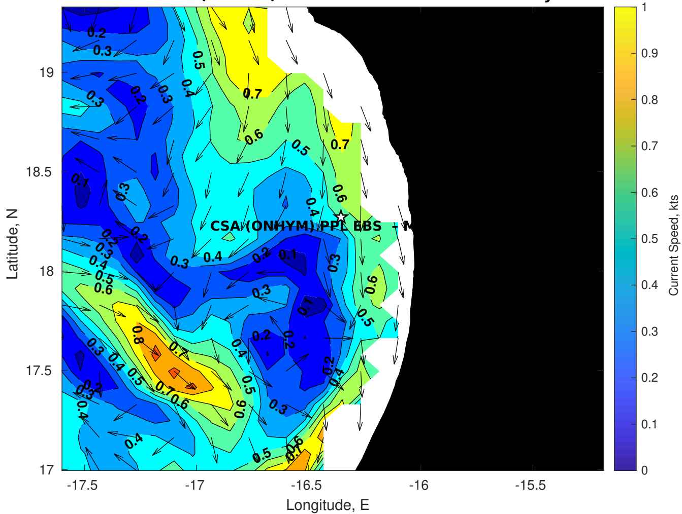
Surface Currents for CSA (ONHYM) PPL EBS - Mauritania at 20-May-2025 00:00:00
