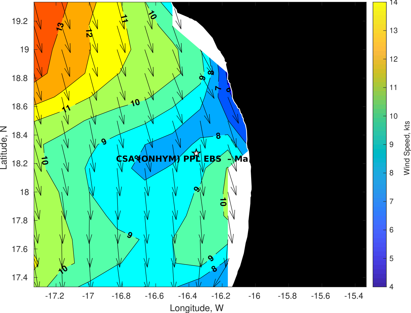
Winds (kts) for CSA (ONHYM) PPL EBS - Mauritania at 21-May-2025 09:00:00
