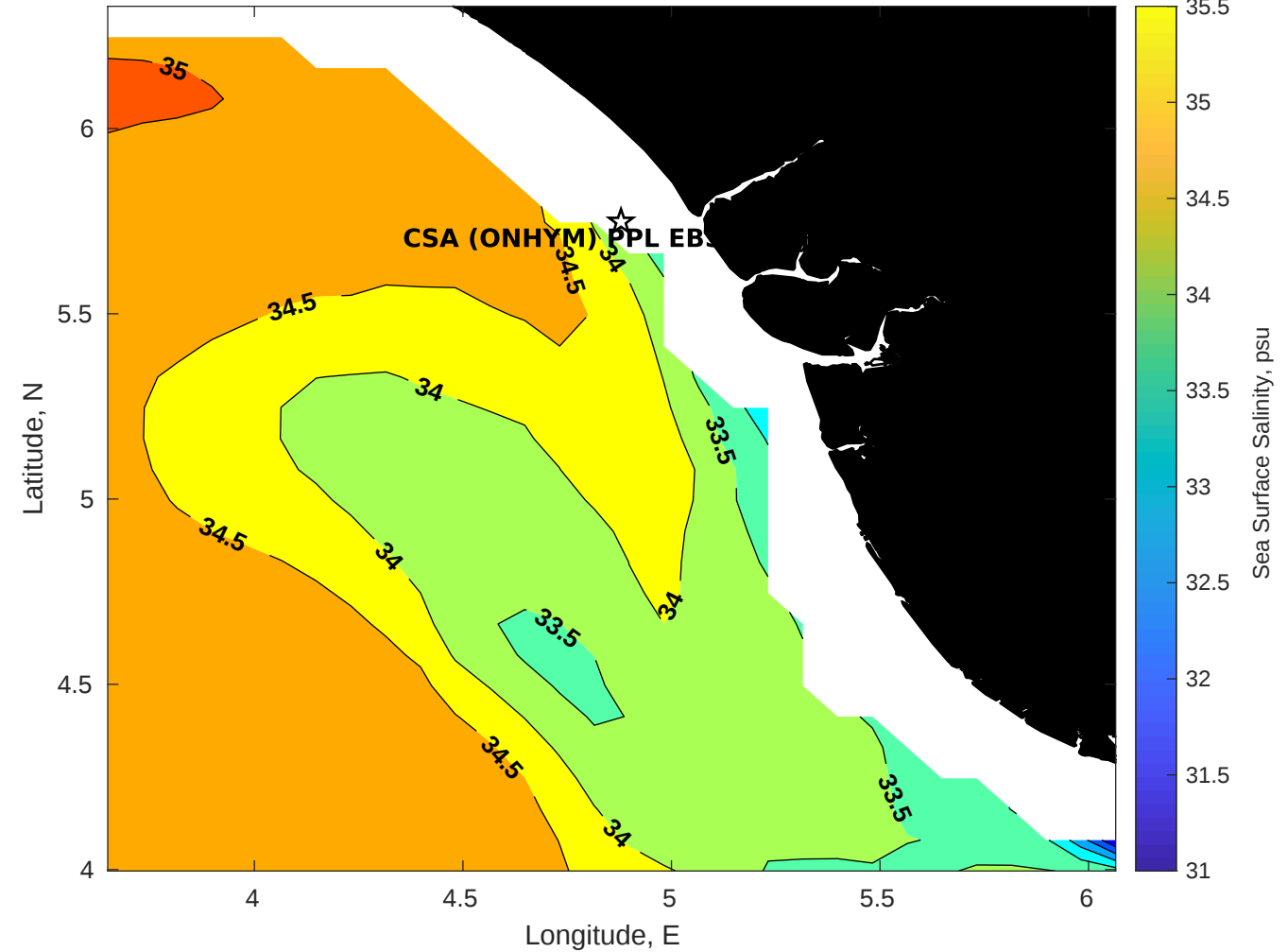
Surface Salinity for CSA (ONHYM) PPL EBS - Nigeria at 20-May-2025 00:00:00
