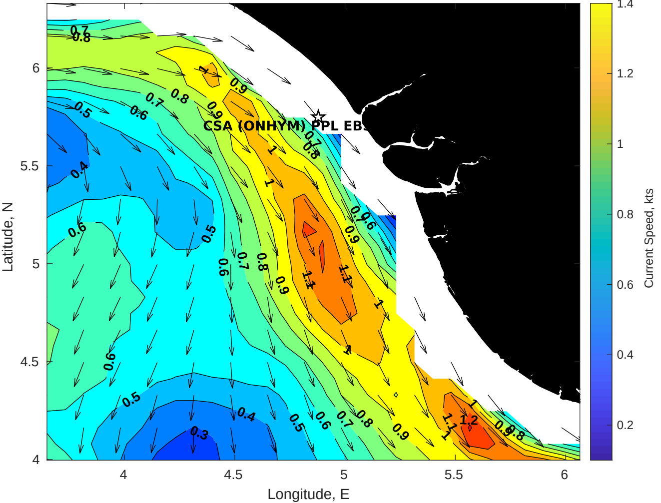
Surface Currents for CSA (ONHYM) PPL EBS - Nigeria at 20-May-2025 00:00:00
