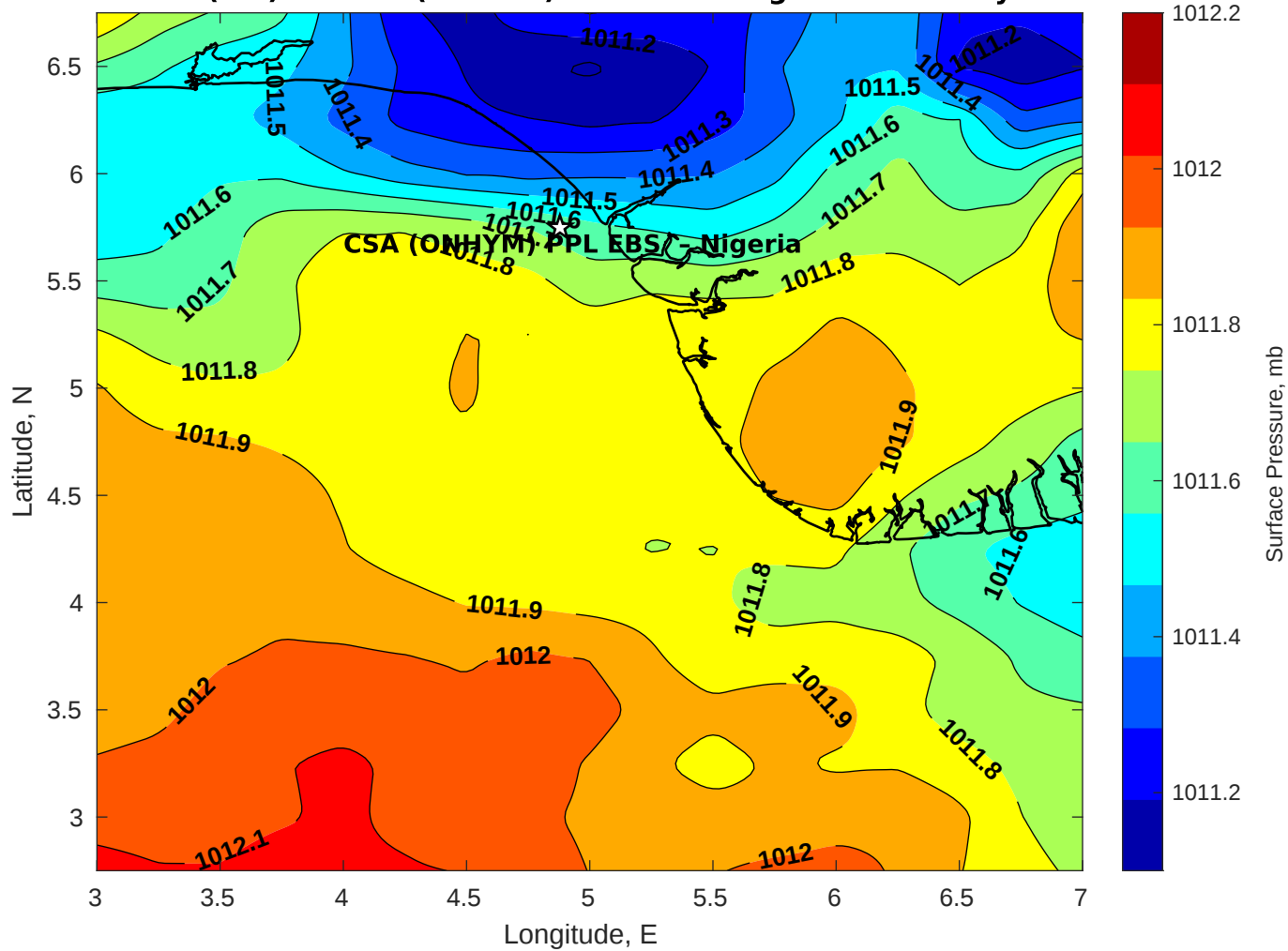
Surface Pressure (mb) for CSA (ONHYM) PPL EBS - Nigeria at 23-May-2025 00:00:00
