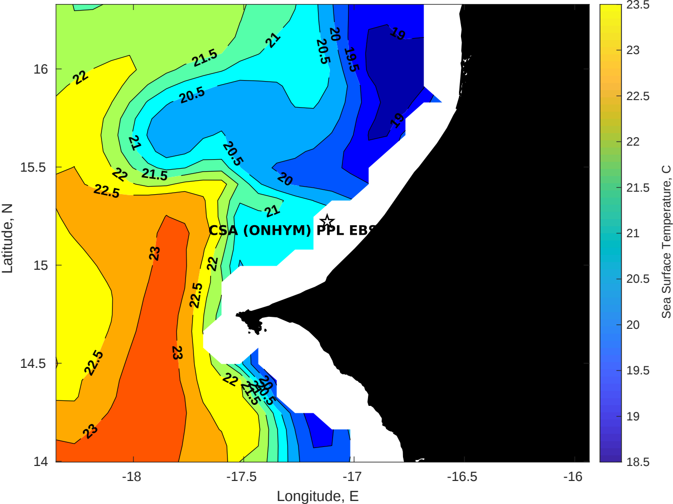
SST for CSA (ONHYM) PPL EBS - Senegal at 20-May-2025 00:00:00
