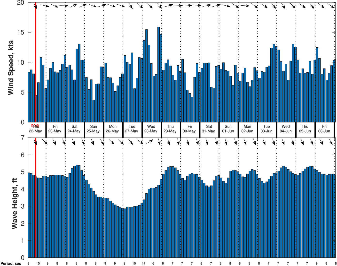
Wind & Wave Forecast for CSA (ONHYM) PPL EBS - Senegal from 21-May-2025 01:00:00 to 06-Jun-2025 01:00:00
