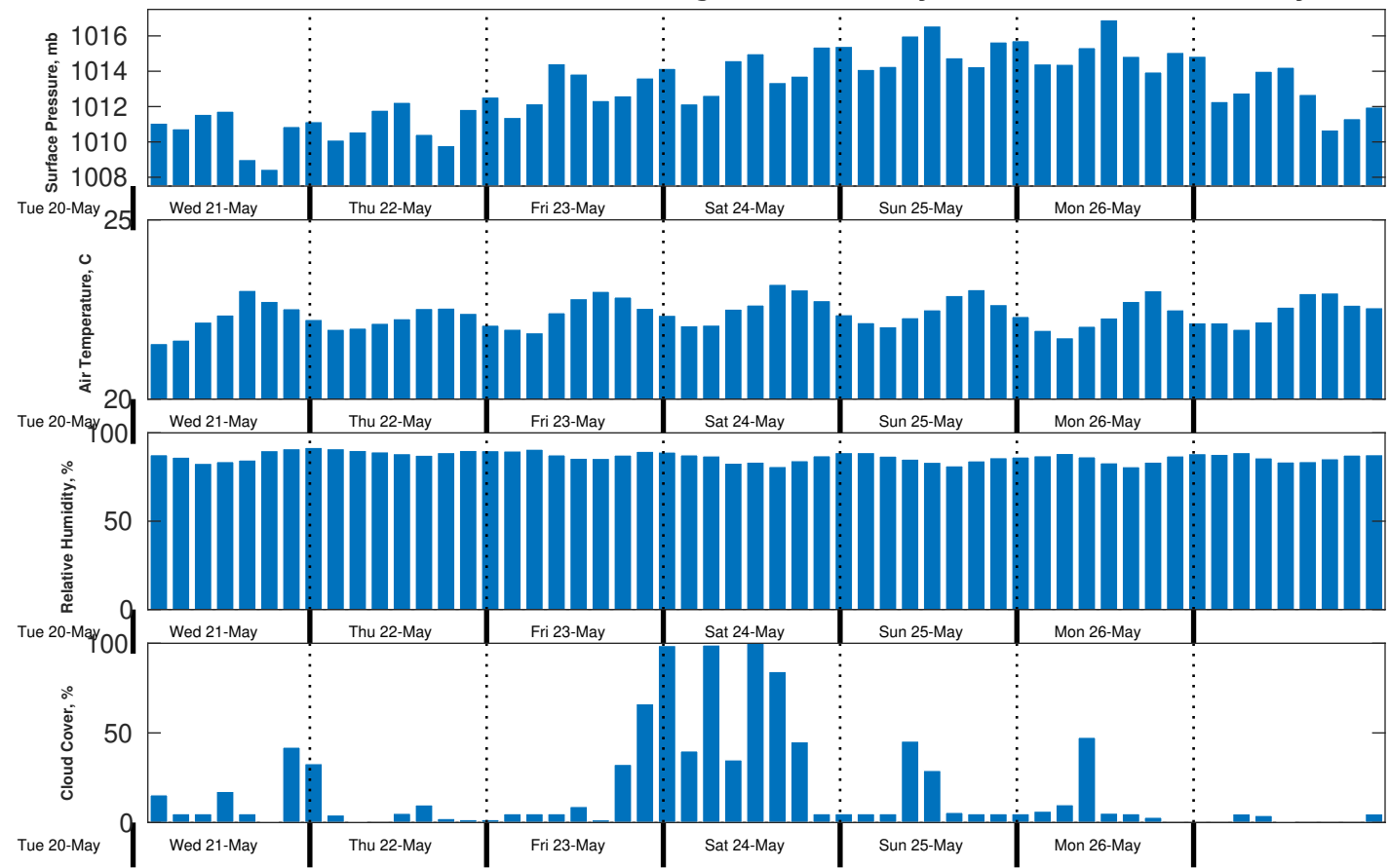
Met Forecast for CSA (ONHYM) PPL EBS - Senegal from 21-May-2025 00:00:00 to 28-May-2025 00:00:00
