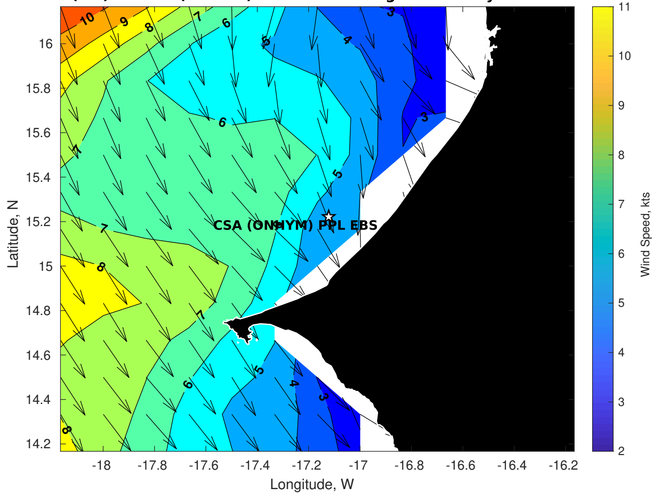
Winds (kts) for CSA (ONHYM) PPL EBS - Senegal at 21-May-2025 09:00:00
