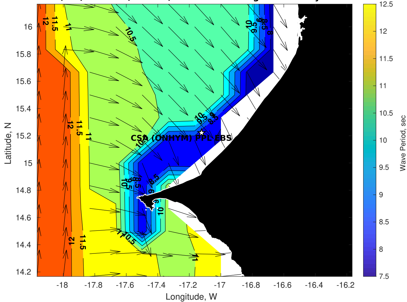
Wave Period (sec) for CSA (ONHYM) PPL EBS - Senegal at 21-May-2025 09:00:00
