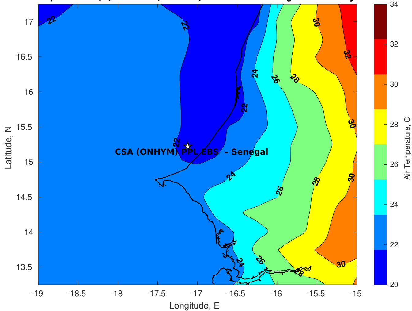
Air Temperature (C) for CSA (ONHYM) PPL EBS - Senegal at 21-May-2025
