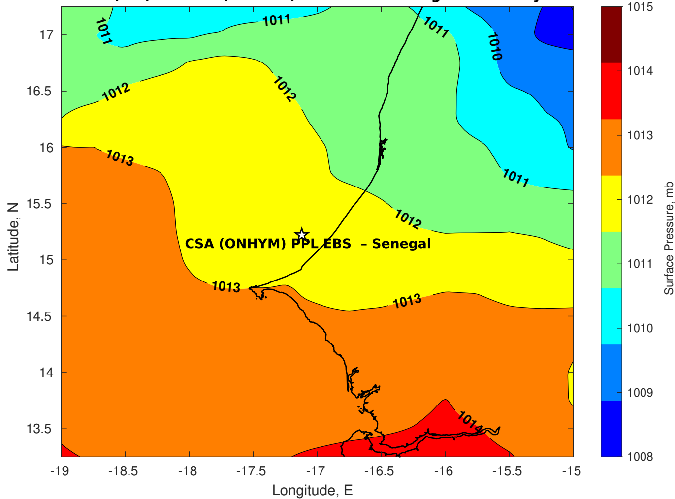
Surface Pressure (mb) for CSA (ONHYM) PPL EBS - Senegal at 23-May-2025 00:00:00
