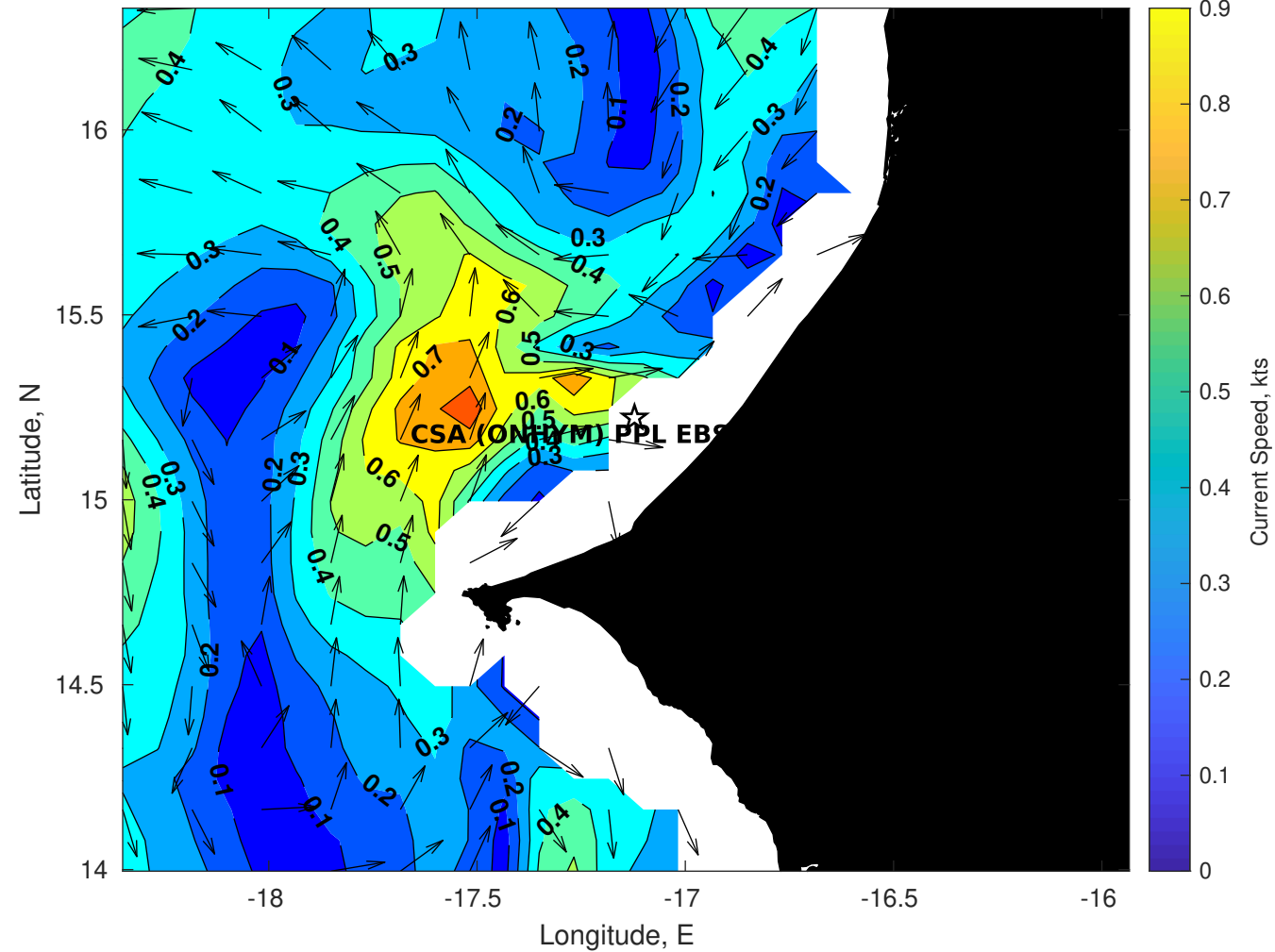
Surface Currents for CSA (ONHYM) PPL EBS - Senegal at 20-May-2025 00:00:00
