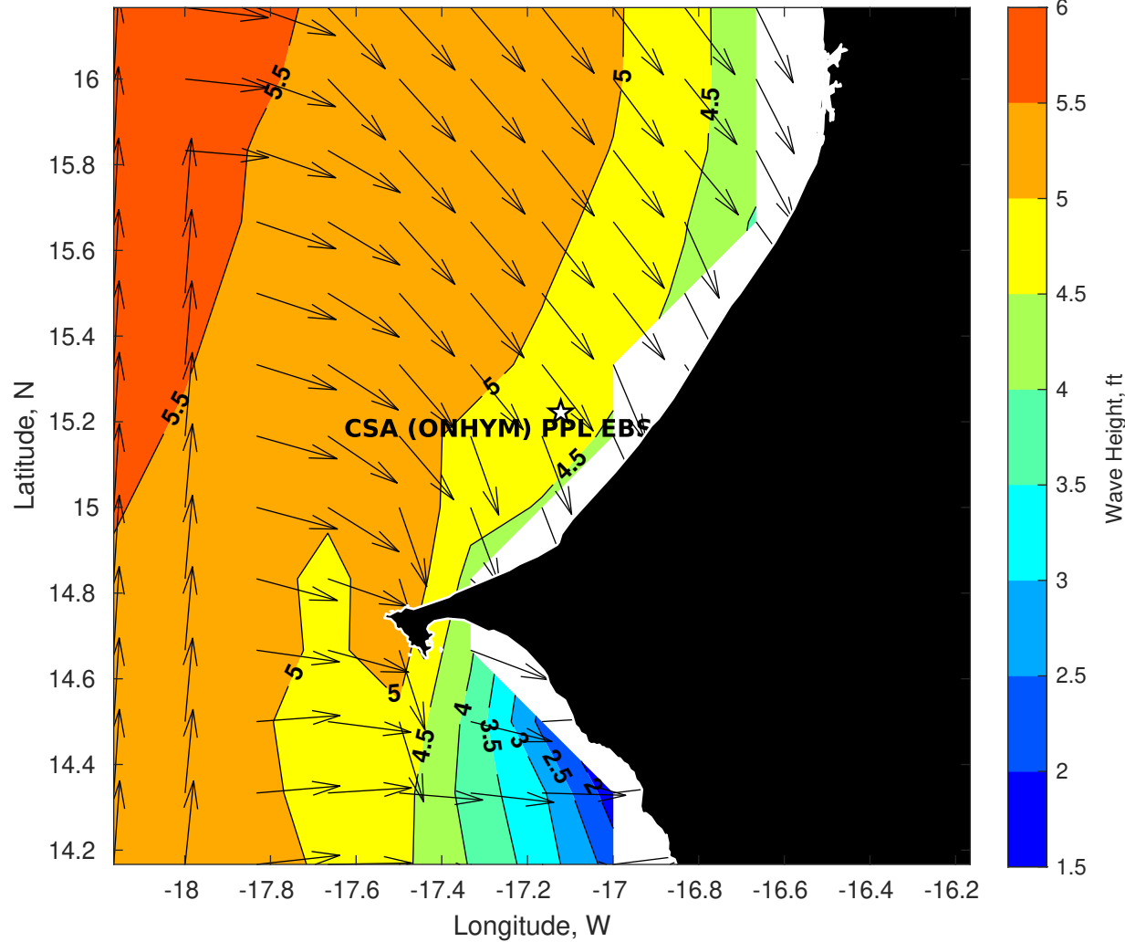
Wave Height (ft) for CSA (ONHYM) PPL EBS - Senegal at 21-May-2025 09:00:00
