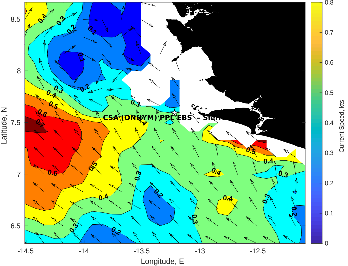
Surface Currents for CSA (ONHYM) PPL EBS - Sierra Leone at 20-May-2025 00:00:00
