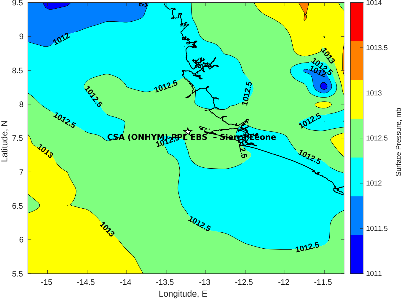
Surface Pressure (mb) for CSA (ONHYM) PPL EBS - Sierra Leone at 22-May-2025 00:00:00
