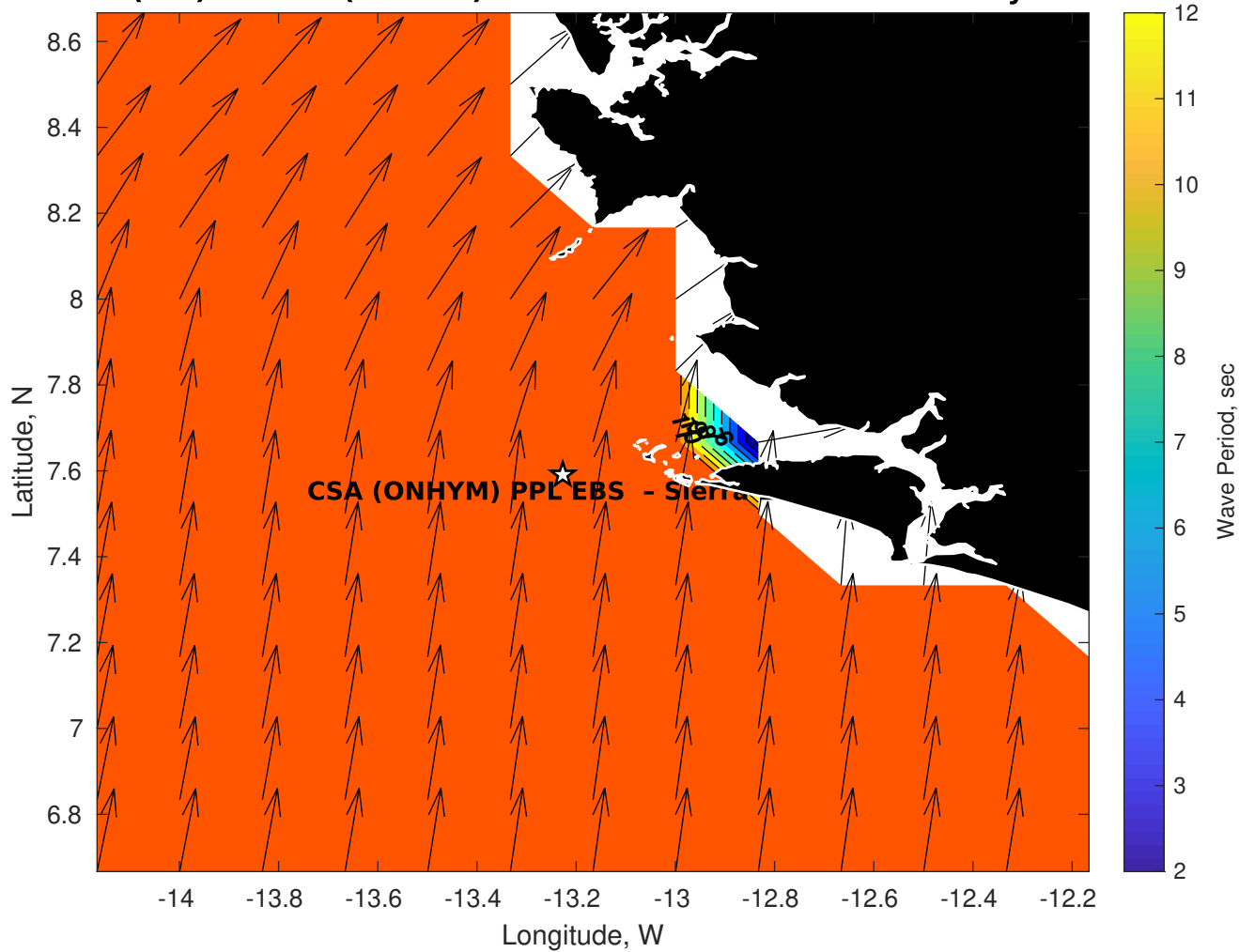
Wave Period (sec) for CSA (ONHYM) PPL EBS - Sierra Leone at 21-May-2025 09:00:00
