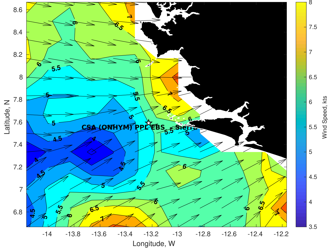
Winds (kts) for CSA (ONHYM) PPL EBS - Sierra Leone at 21-May-2025 09:00:00
