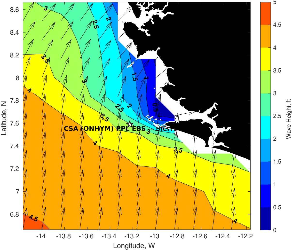
Wave Height (ft) for CSA (ONHYM) PPL EBS - Sierra Leone at 21-May-2025 09:00:00
