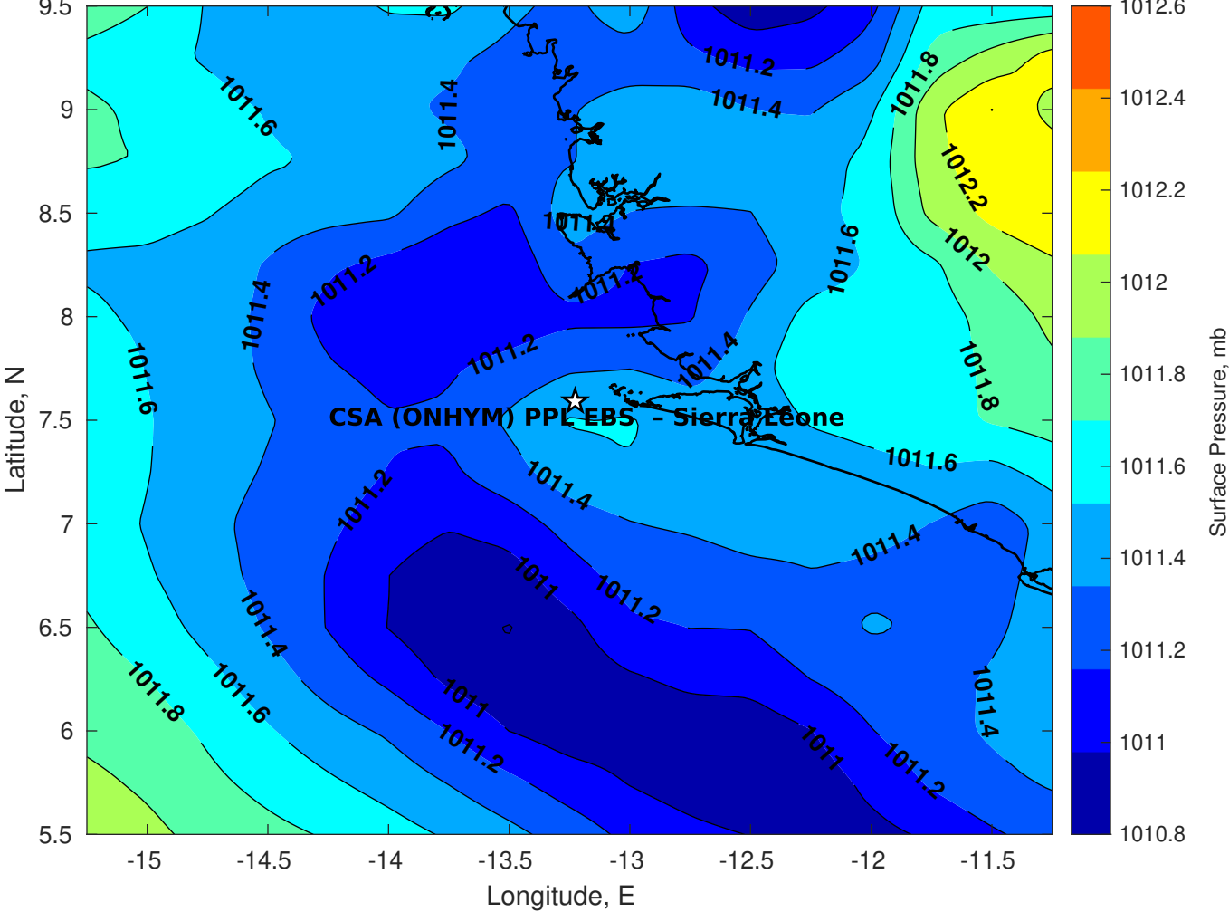
Surface Pressure (mb) for CSA (ONHYM) PPL EBS - Sierra Leone at 21-May-2025 00:00:00
