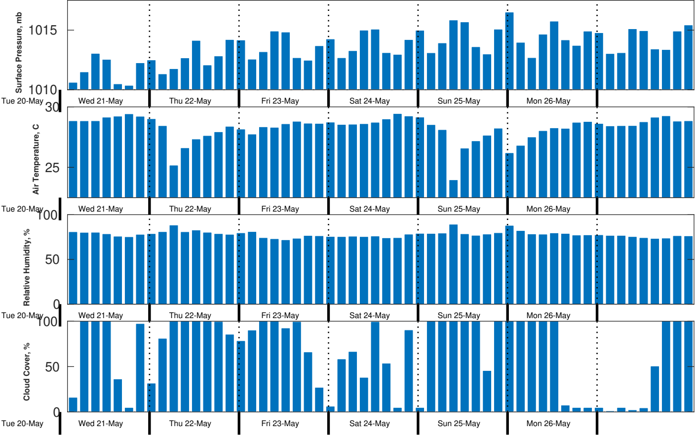
Met Forecast for CSA (ONHYM) PPL EBS - Sierra Leone from 21-May-2025 00:00:00 to 28-May-2025 00:00:00
