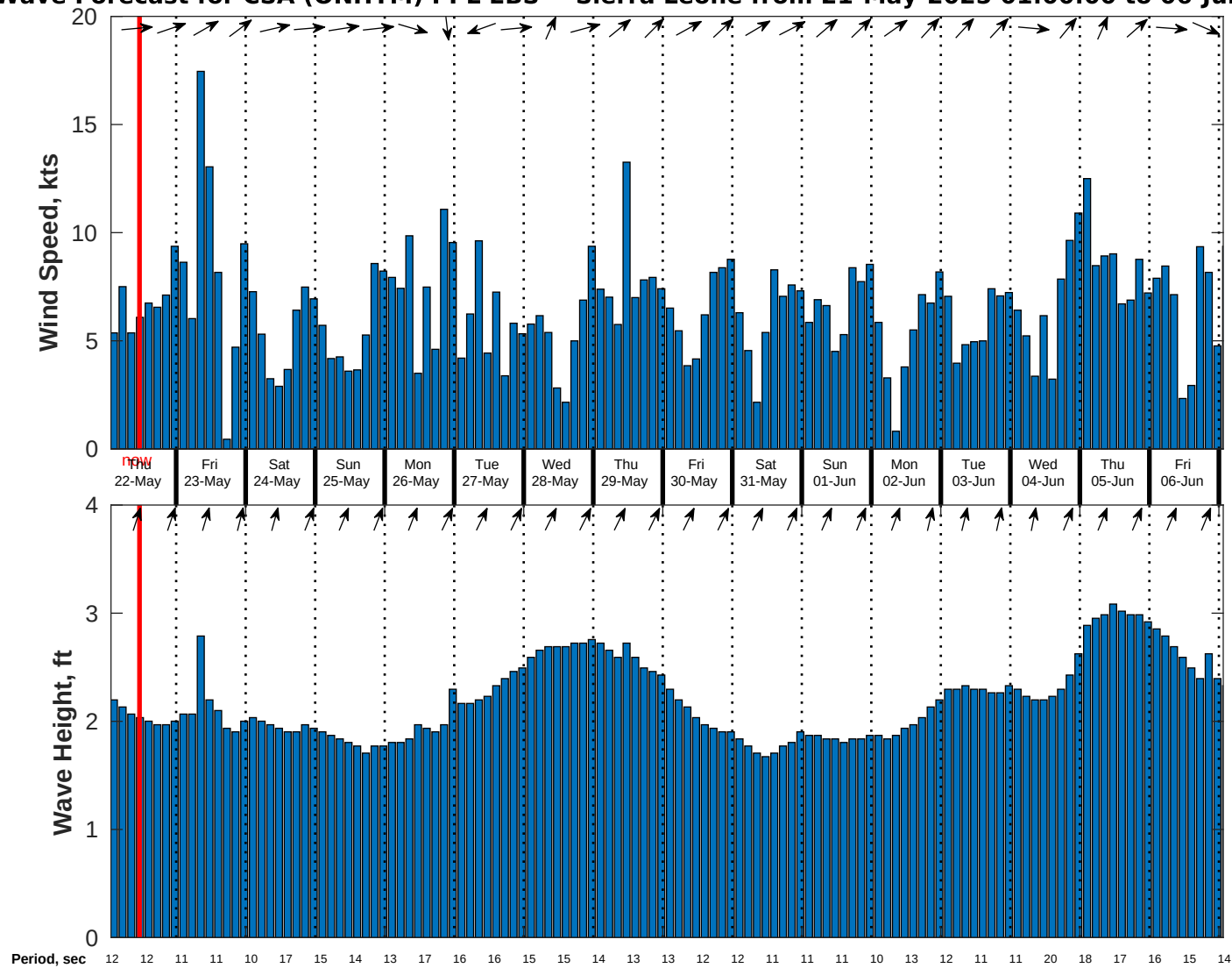
Wind & Wave Forecast for CSA (ONHYM) PPL EBS - Sierra Leone from 21-May-2025 01:00:00 to 06-Jun-2025 01:00:00
