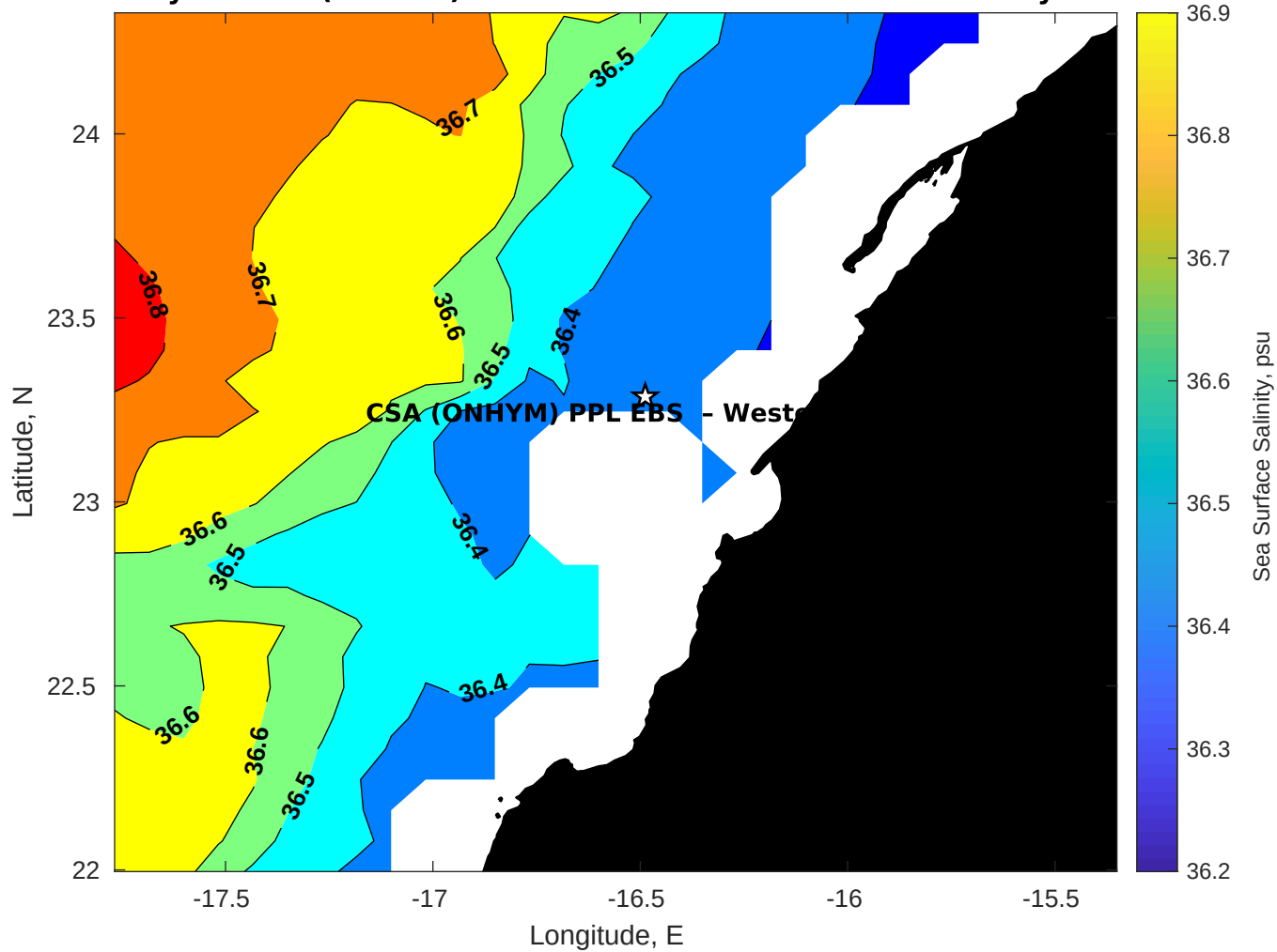
Surface Salinity for CSA (ONHYM) PPL EBS - Western Sahara at 20-May-2025 00:00:00
