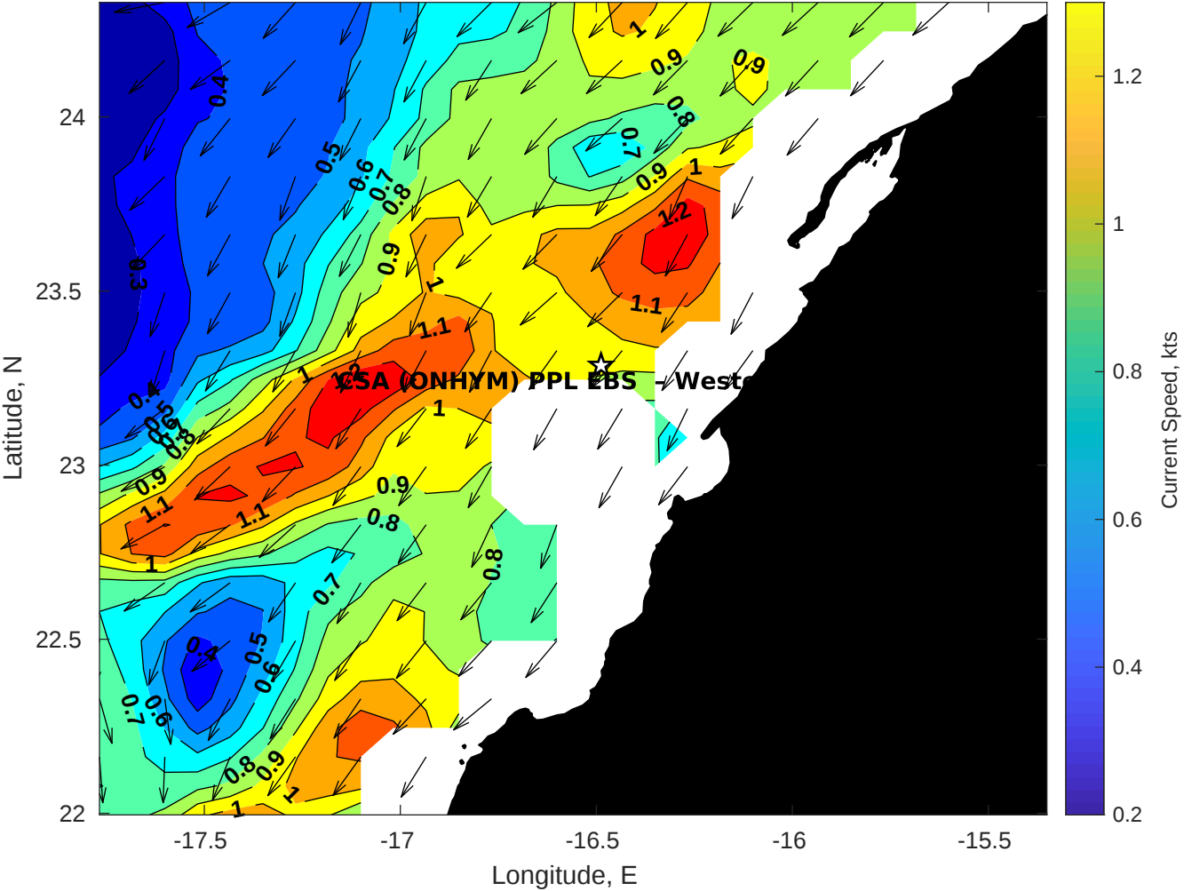
Surface Currents for CSA (ONHYM) PPL EBS - Western Sahara at 20-May-2025 00:00:00
