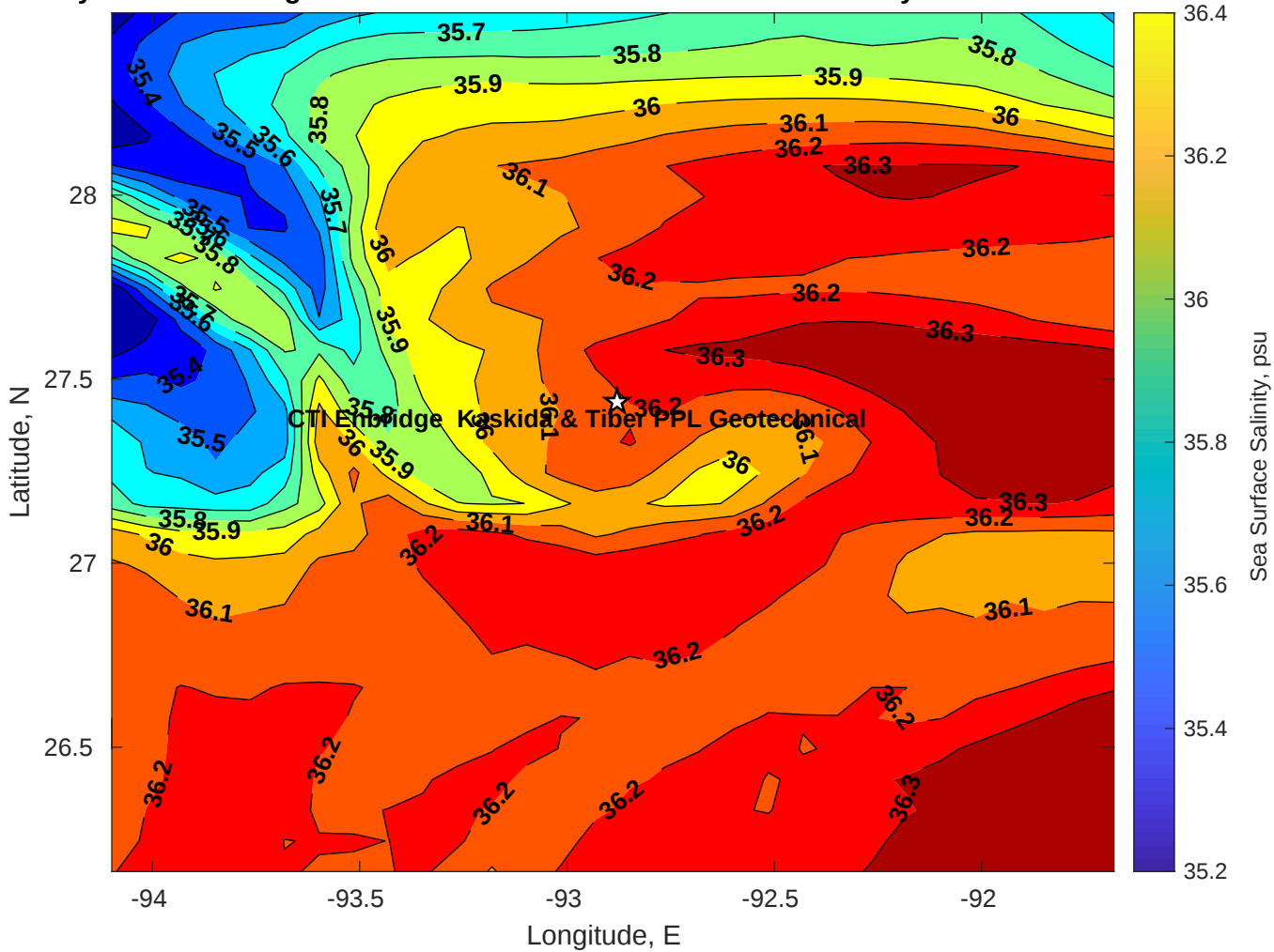
Surface Salinity for CTI Enbridge Kaskida & Tiber PPL Geotechnical at 20-May-2025 00:00:00
