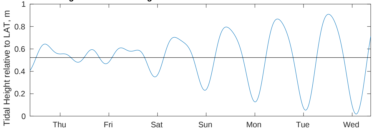
Tidal Currents and Heights for CTI Enbridge Kaskida & Tiber PPL Geotechnical at 20250521
