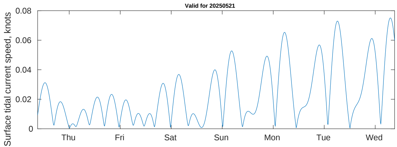
Tidal Currents and Heights for CTI Enbridge Kaskida & Tiber PPL Geotechnical at 20250521
