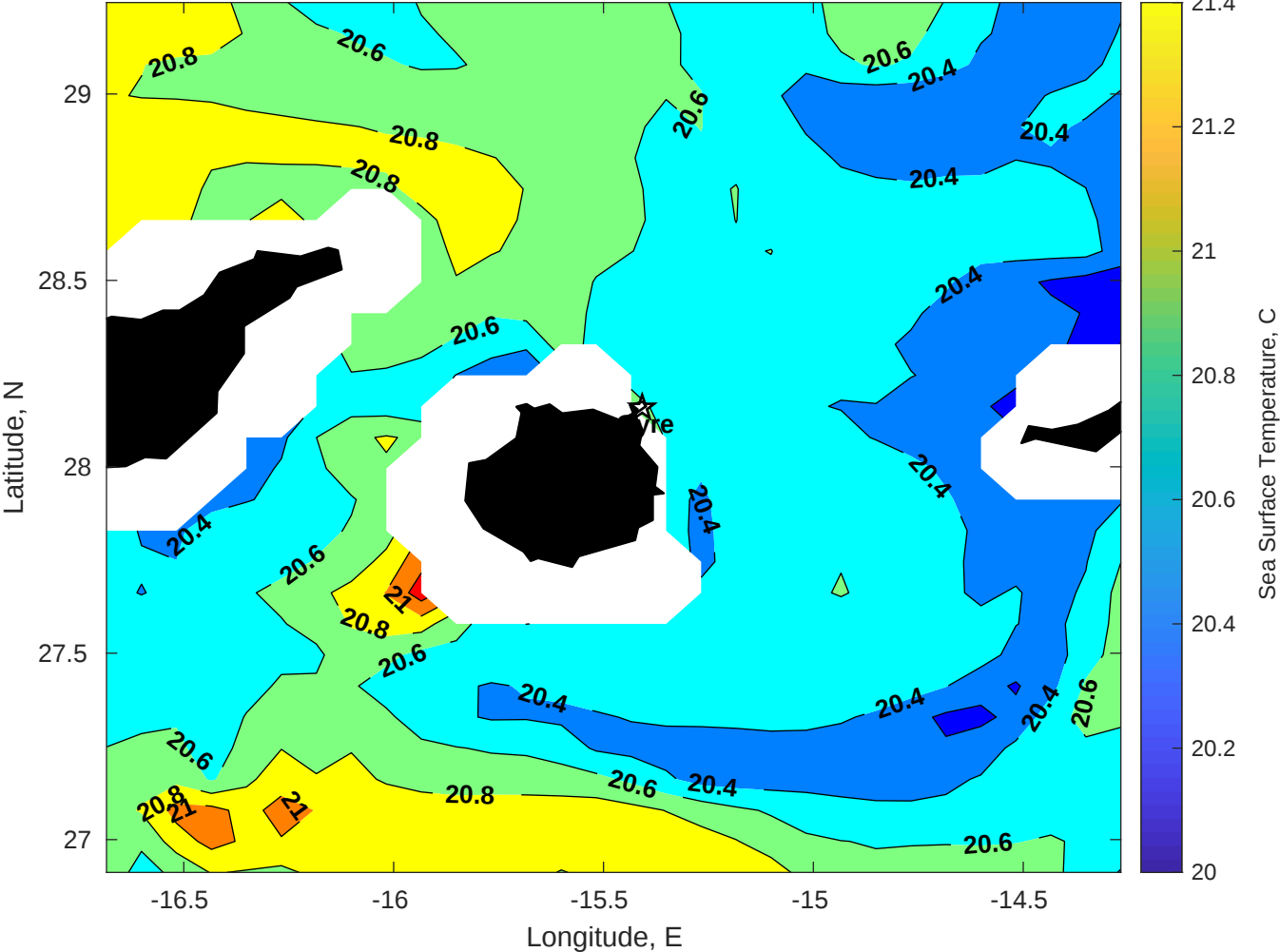
SST for Gyre at 20-May-2025 00:00:00
