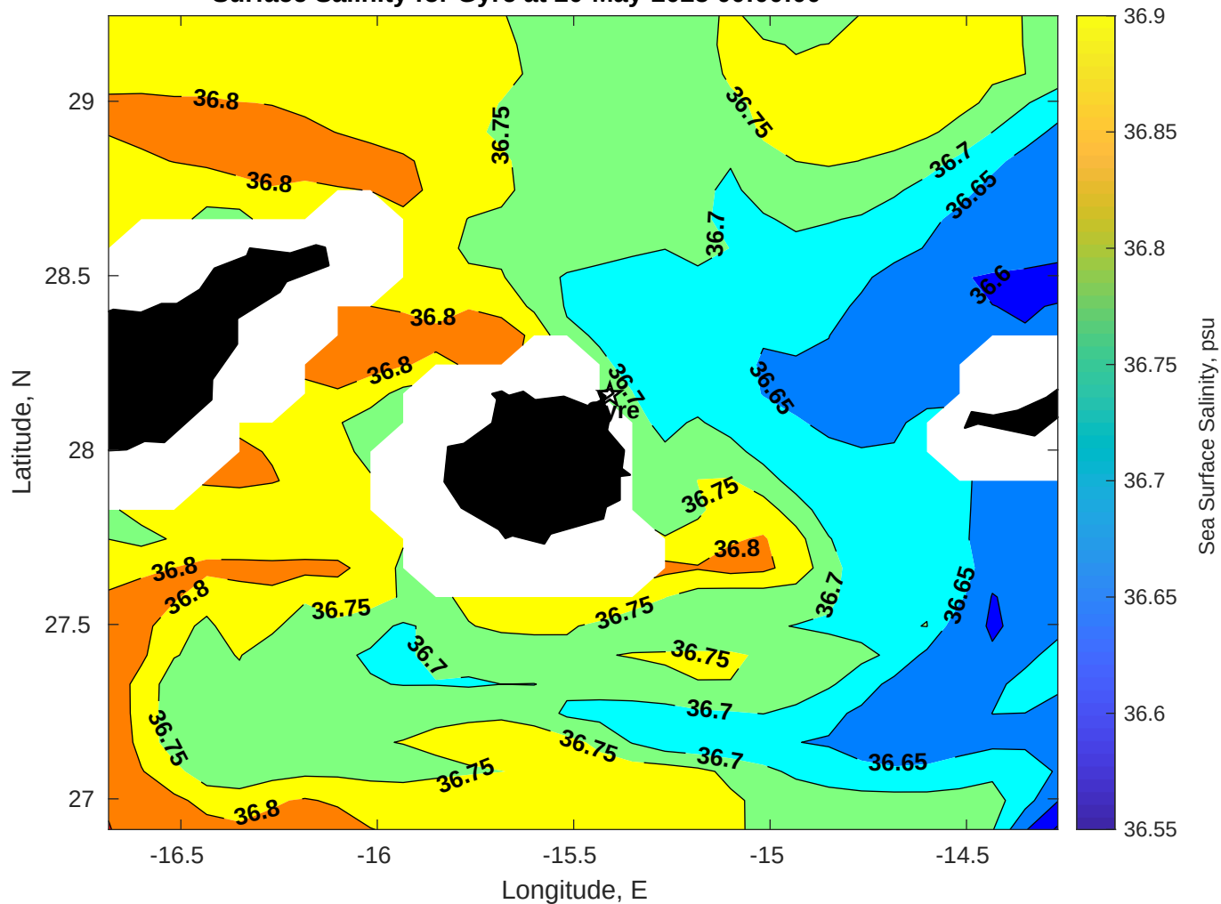
Surface Salinity for Gyre at 20-May-2025 00:00:00
