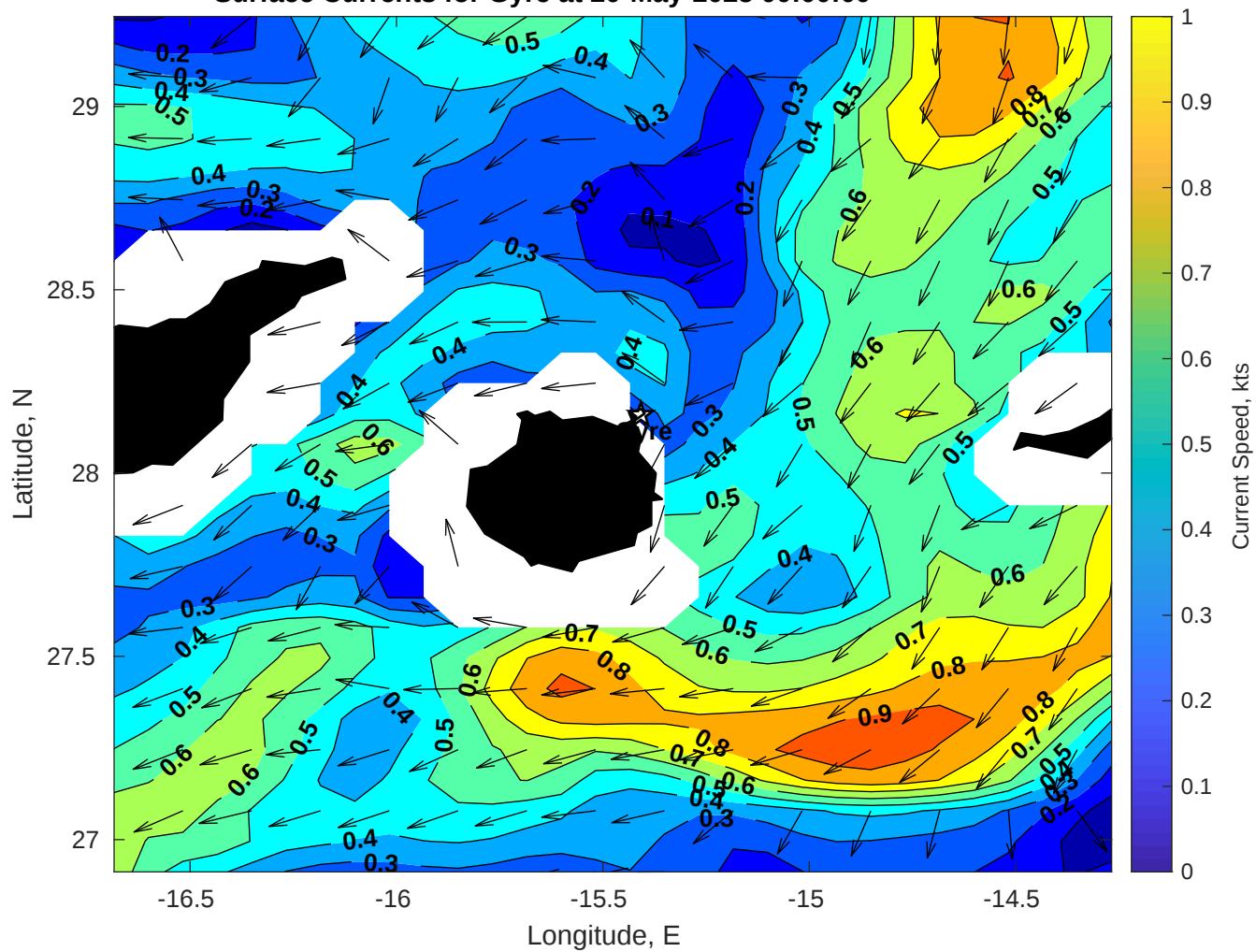
Surface Currents for Gyre at 20-May-2025 00:00:00
