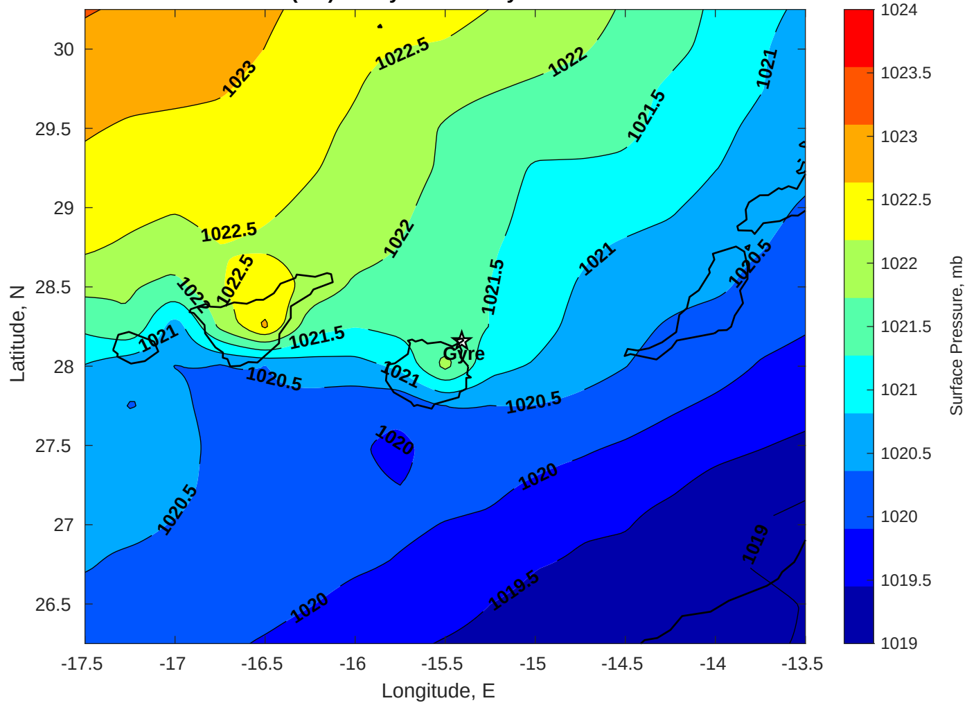
Surface Pressure (mb) for Gyre at 21-May-2025 00:00:00
