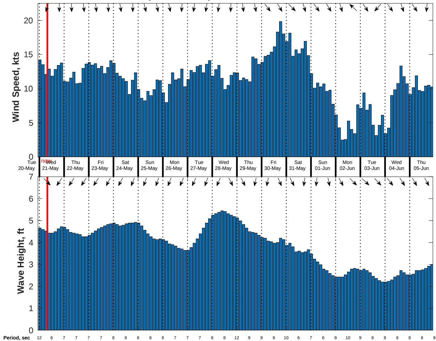
Wind & Wave Forecast for Gyre from 20-May-2025 23:00:00 to 05-Jun-2025 23:00:00
