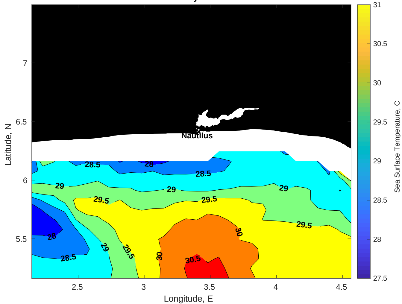
SST for Nautilus at 20-May-2025 00:00:00
