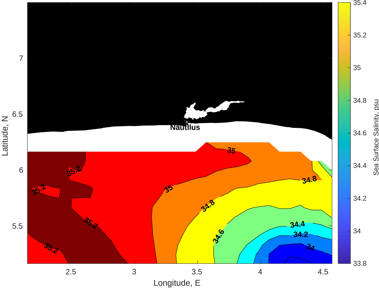
Surface Salinity for Nautilus at 20-May-2025 00:00:00
