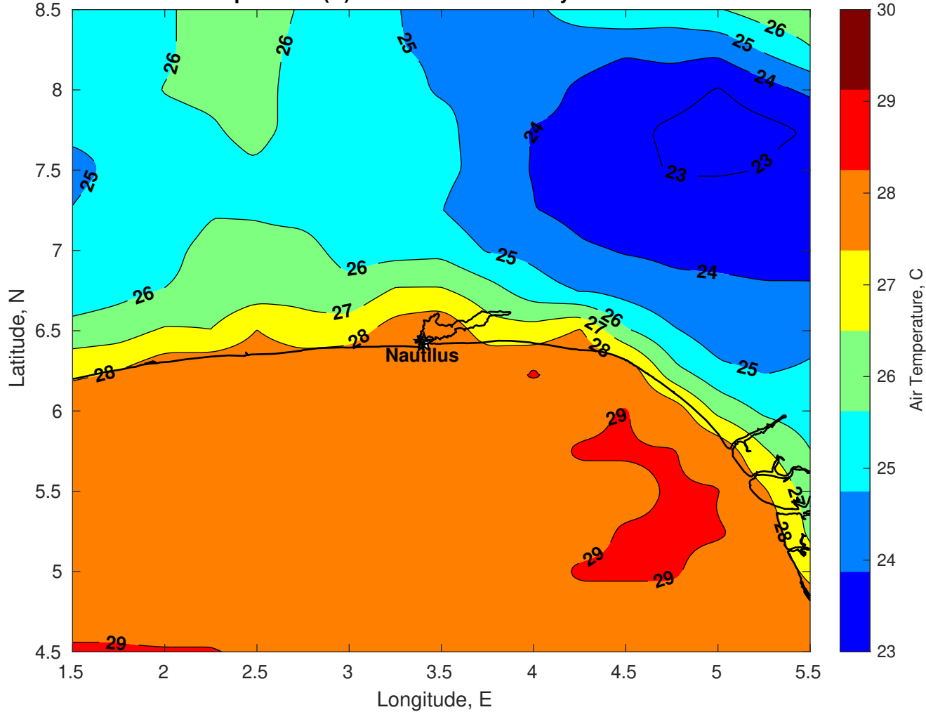
Air Temperature (C) for Nautilus at 21-May-2025
