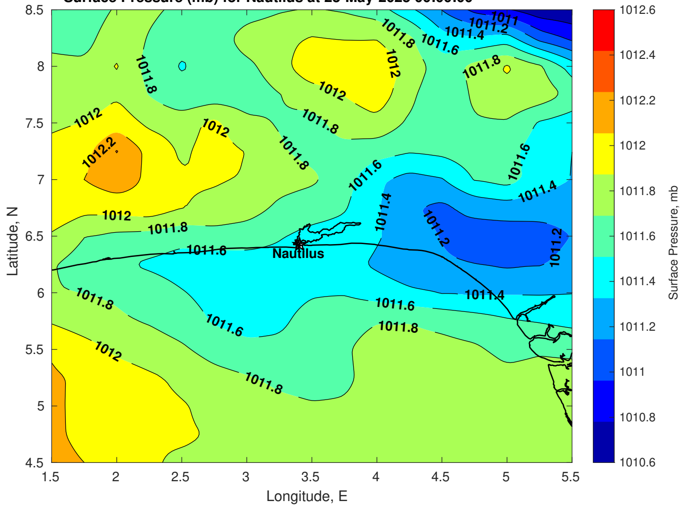
Surface Pressure (mb) for Nautilus at 23-May-2025 00:00:00
