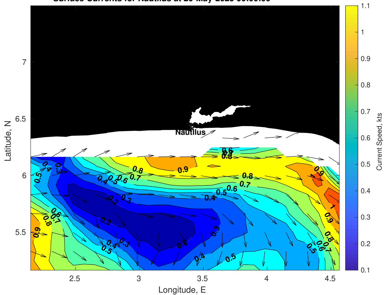
Surface Currents for Nautilus at 20-May-2025 00:00:00
