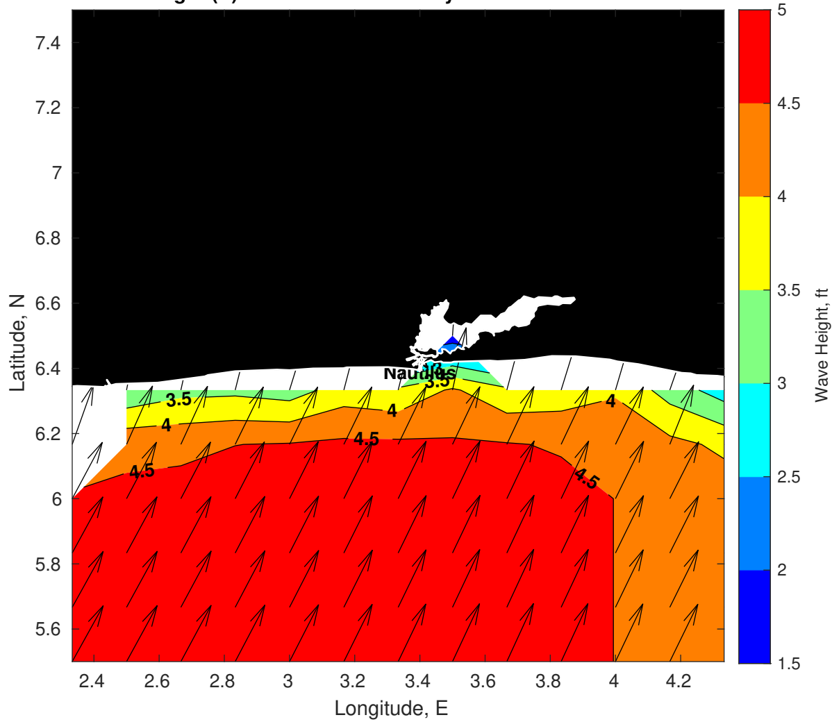
Wave Height (ft) for Nautilus at 21-May-2025 09:00:00
