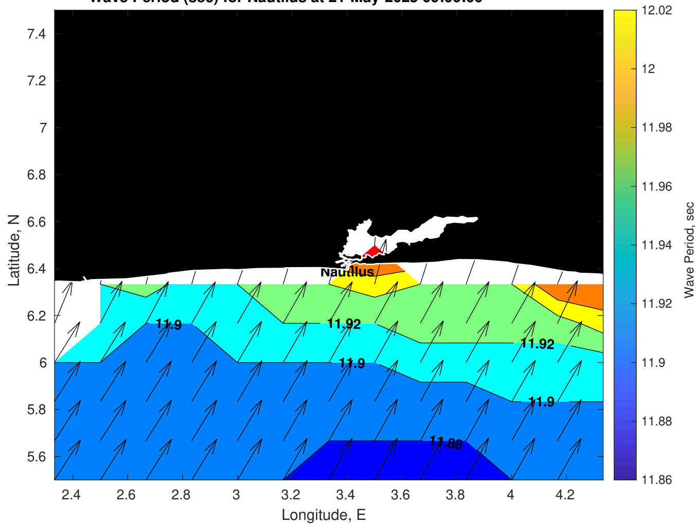
Wave Period (sec) for Nautilus at 21-May-2025 09:00:00
