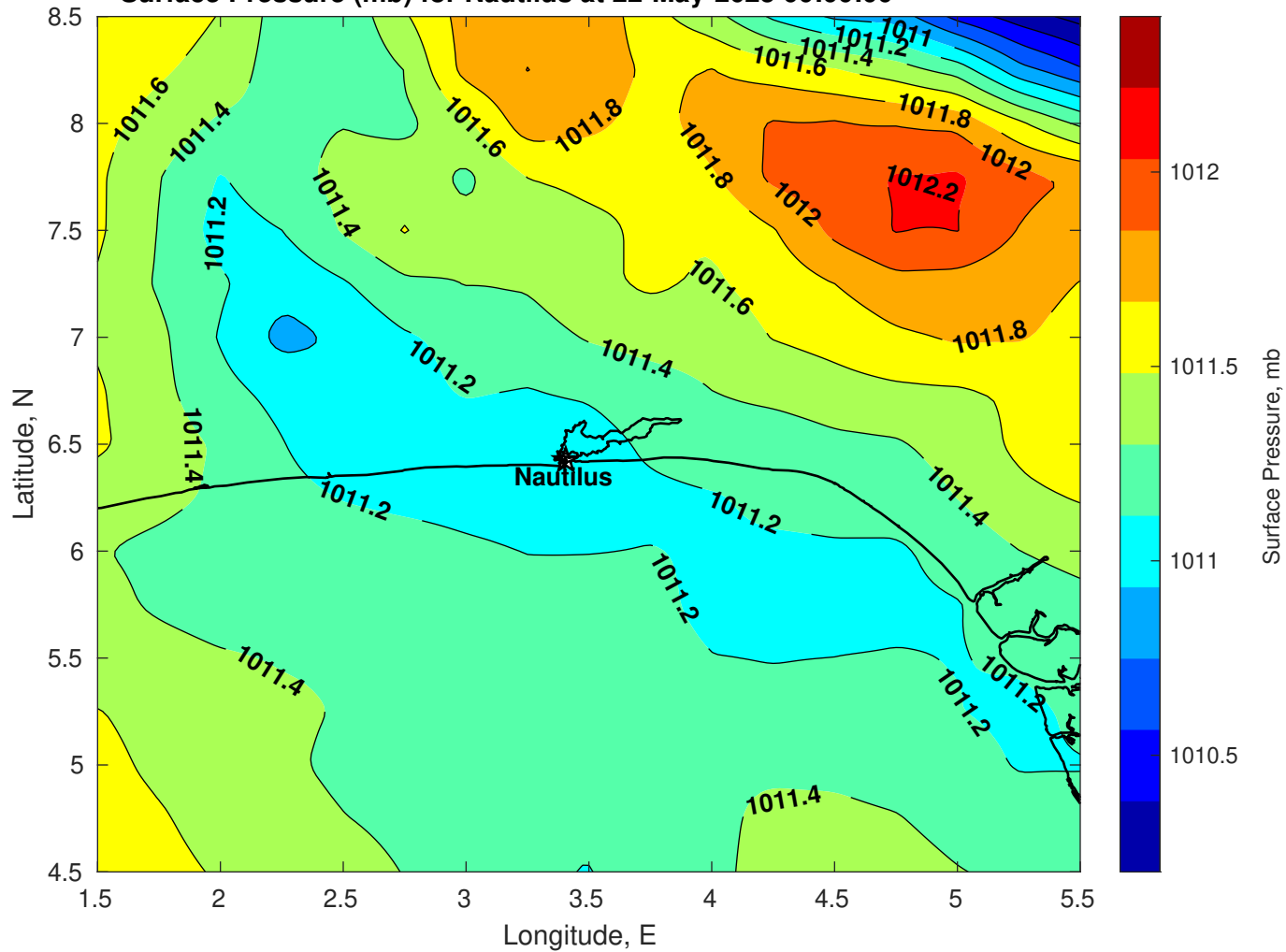
Surface Pressure (mb) for Nautilus at 22-May-2025 00:00:00
