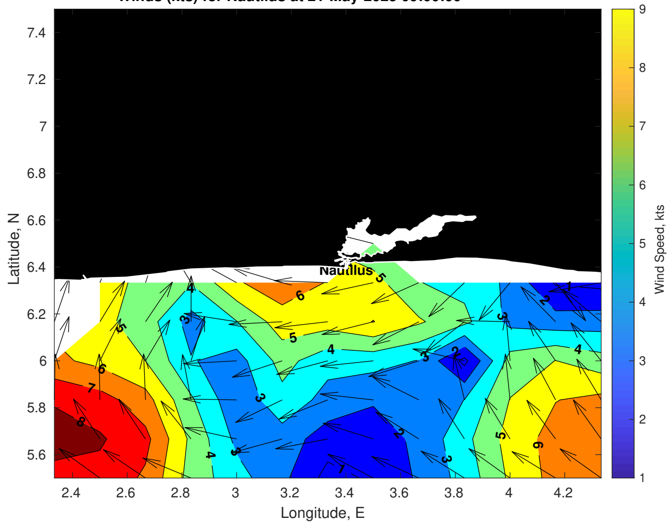
Winds (kts) for Nautilus at 21-May-2025 09:00:00
