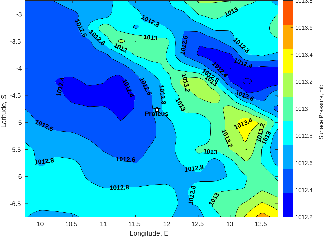
Surface Pressure (mb) for Proteus at 22-May-2025 00:00:00
