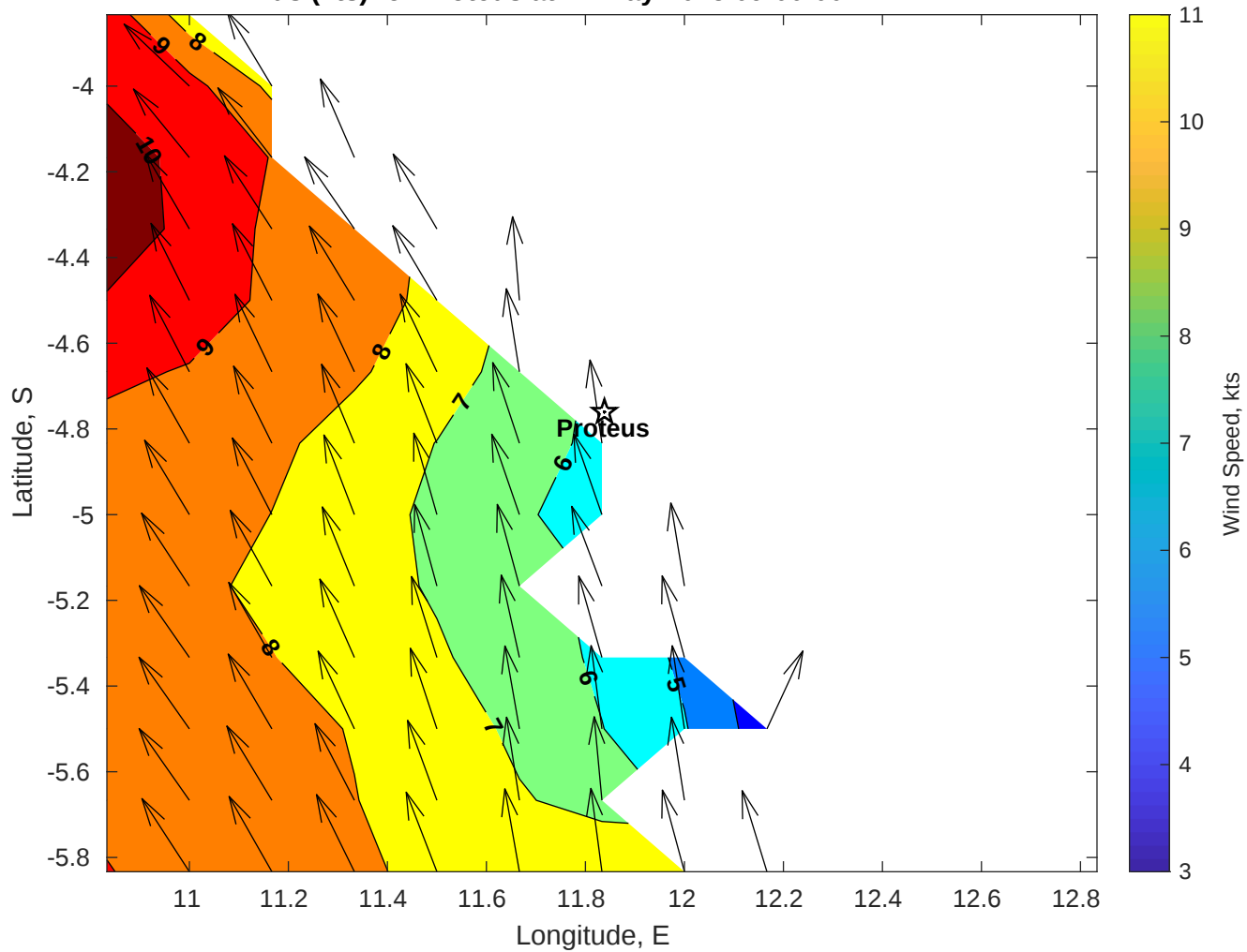
Winds (kts) for Proteus at 21-May-2025 09:00:00
