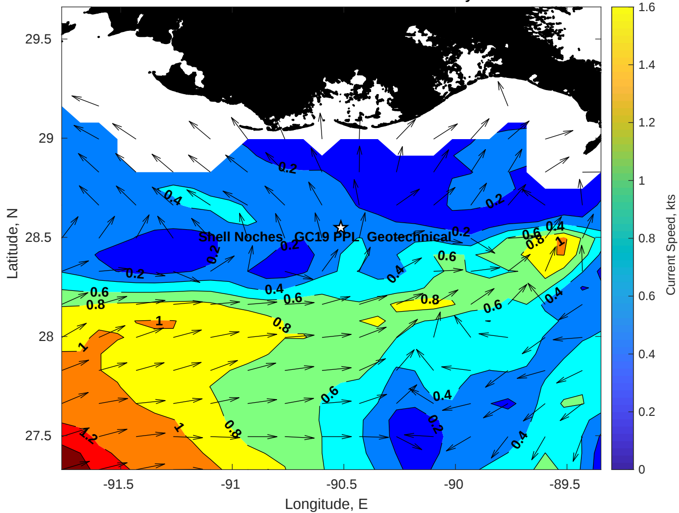
Surface Currents for Shell Noches GC19 PPL Geotechnical at 20-May-2025 00:00:00
