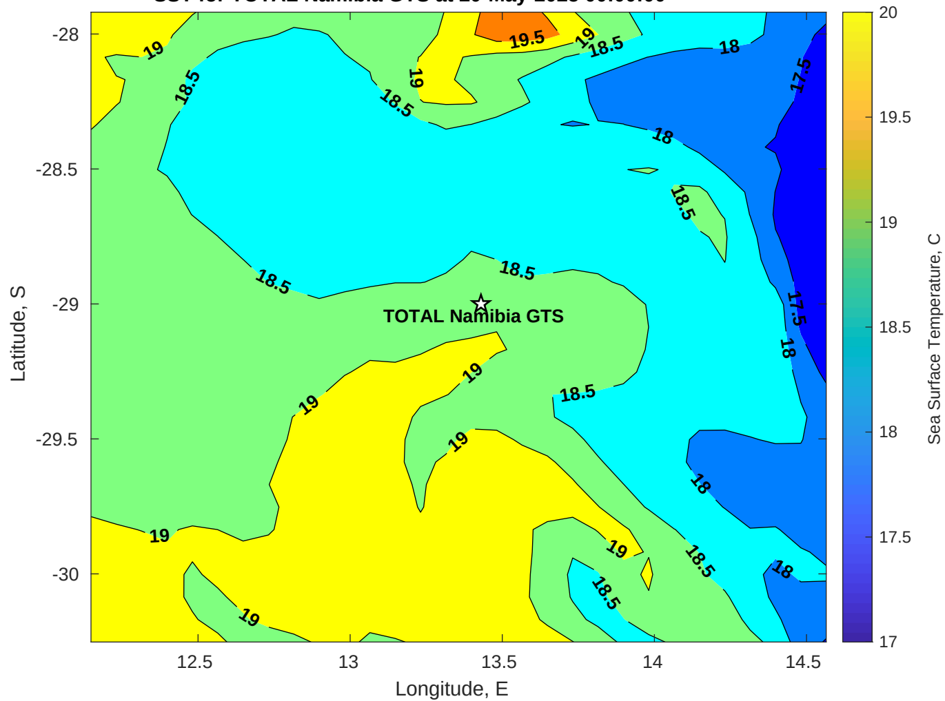
SST for TOTAL Namibia GTS at 20-May-2025 00:00:00
