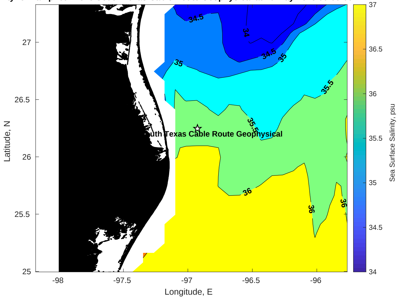
Surface Salinity for Tampnet P2378 South Texas Cable Route Geophysical at 20-May-2025 00:00:00
