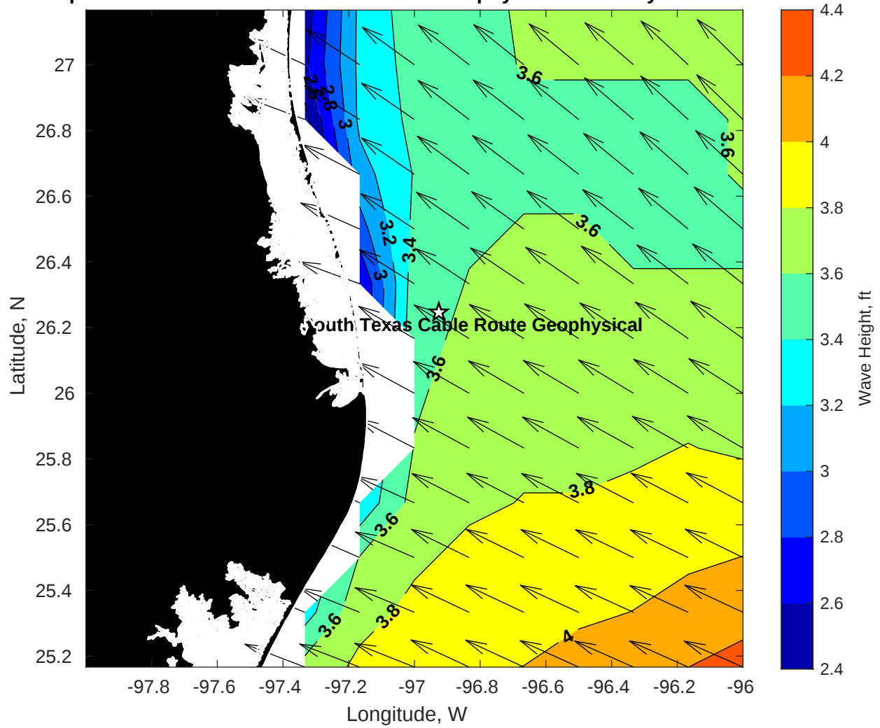
Wave Height (ft) for Tampnet P2378 South Texas Cable Route Geophysical at 21-May-2025 09:00:00
