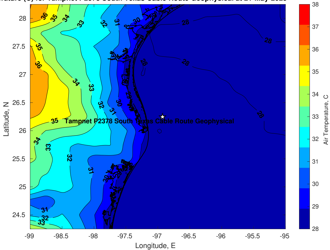
Air Temperature (C) for Tampnet P2378 South Texas Cable Route Geophysical at 21-May-2025
