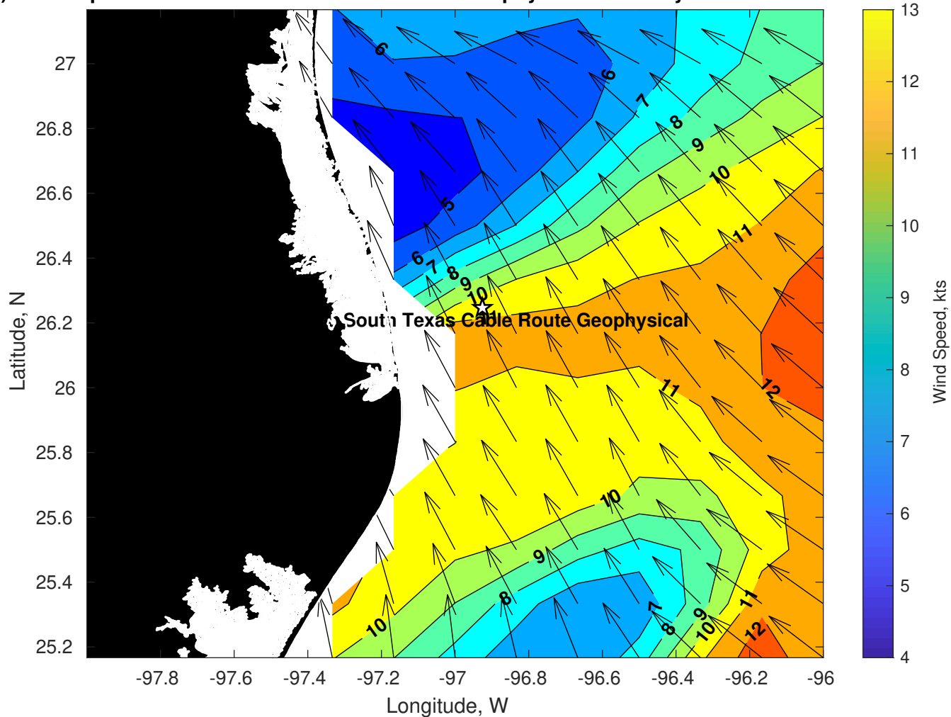
Winds (kts) for Tampnet P2378 South Texas Cable Route Geophysical at 21-May-2025 09:00:00
