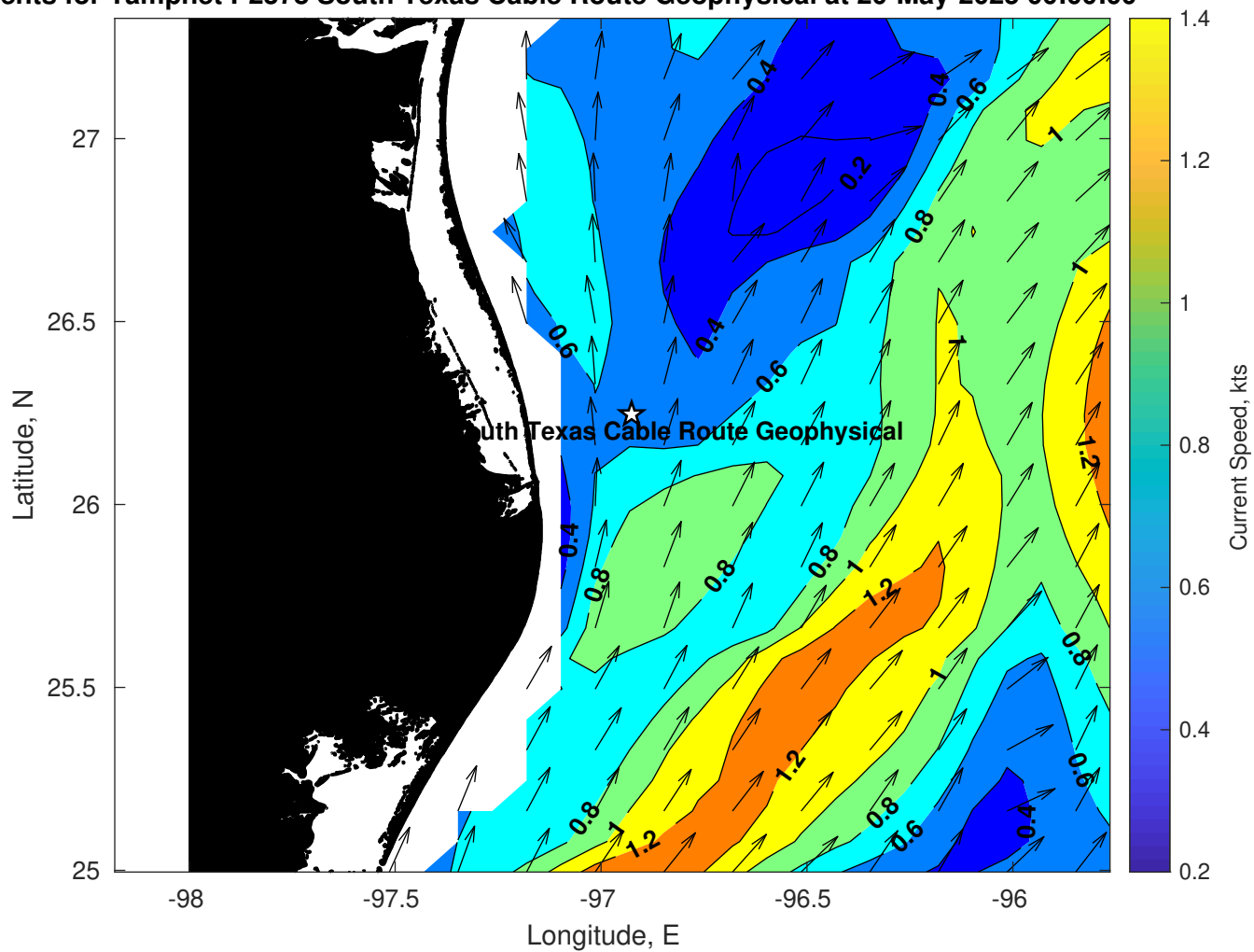
Surface Currents for Tampnet P2378 South Texas Cable Route Geophysical at 20-May-2025 00:00:00
