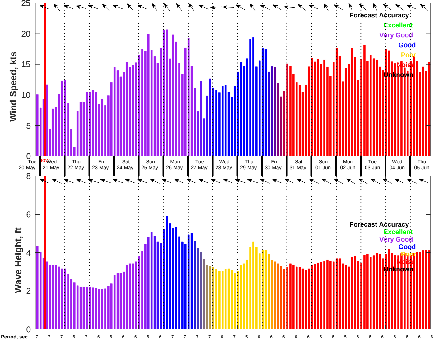
Wind & Wave Forecast for Tampnet P2378 South Texas Cable Route Geophysical from 20-May-2025 20:00:00 to 05-Jun-2025 20:00:00
