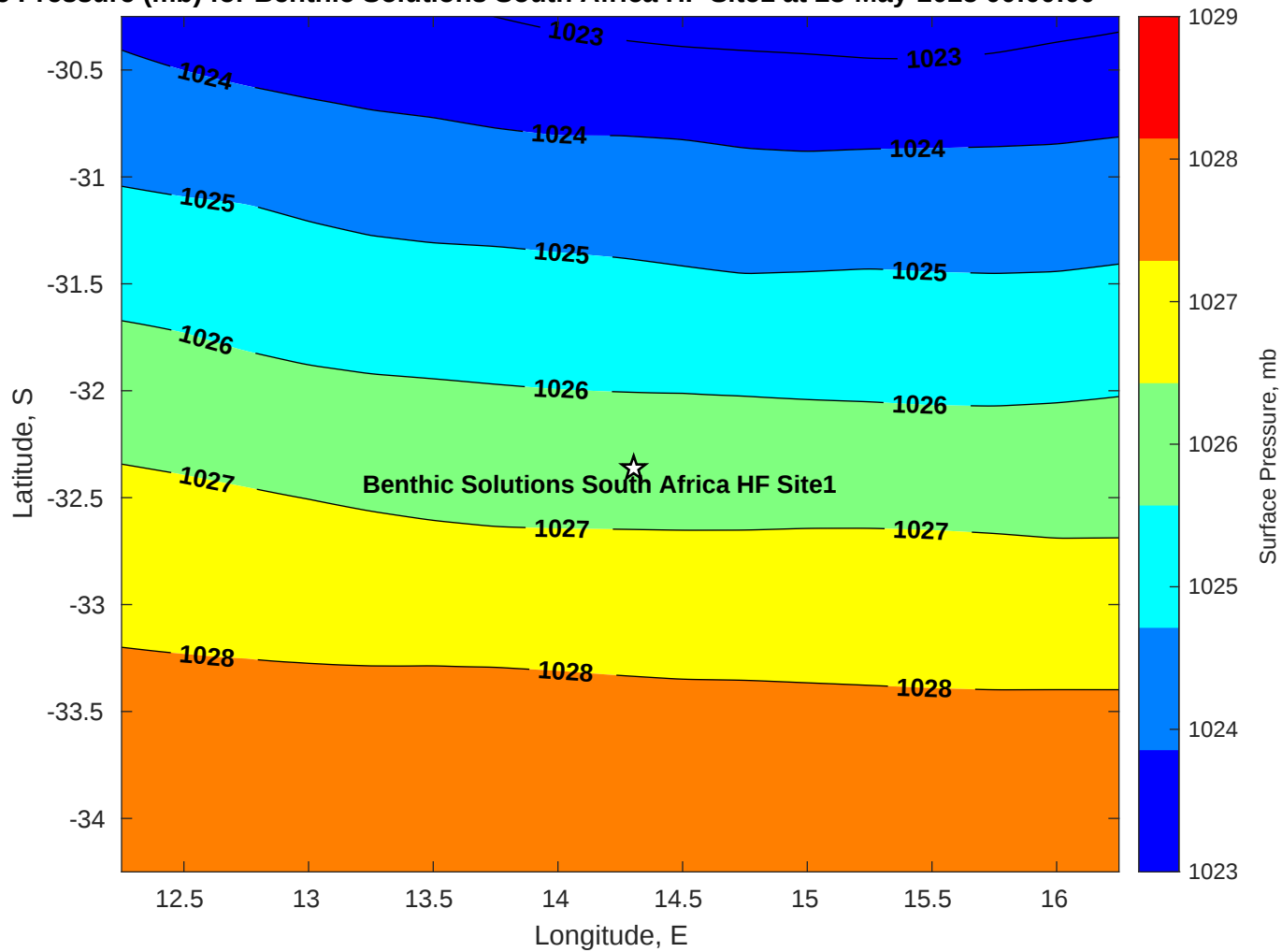
Surface Pressure (mb) for Benthic Solutions South Africa HF Site1 at 23-May-2025 00:00:00
