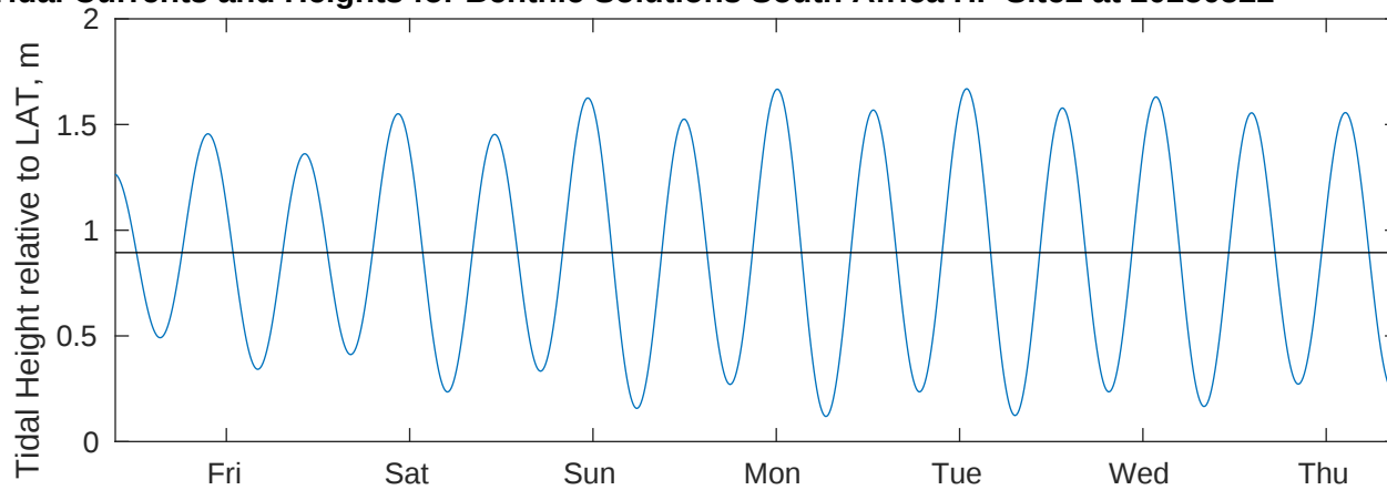
Tidal Currents and Heights for Benthic Solutions South Africa HF Site2 at 20250522
