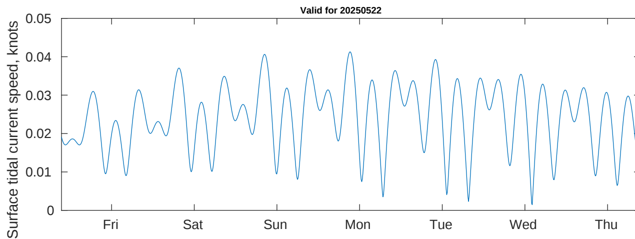
Tidal Currents and Heights for Benthic Solutions South Africa HF Site2 at 20250522
