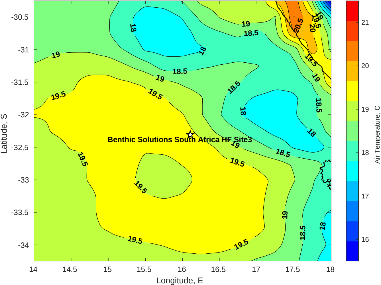
Air Temperature (C) for Benthic Solutions South Africa HF Site3 at 22-May-2025
