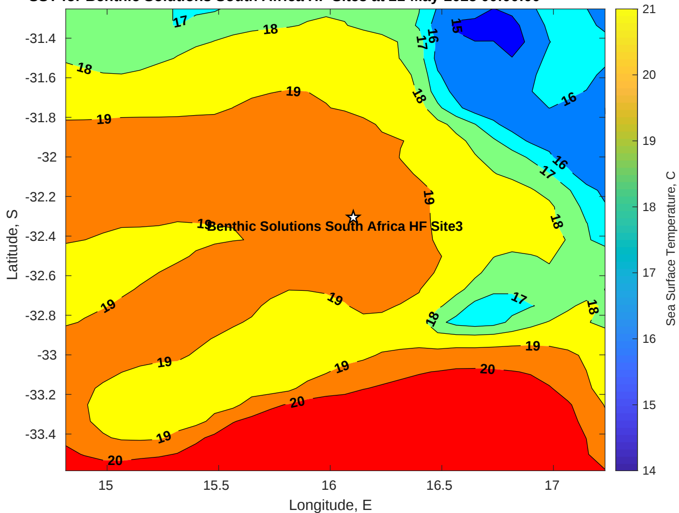
SST for Benthic Solutions South Africa HF Site3 at 21-May-2025 00:00:00
