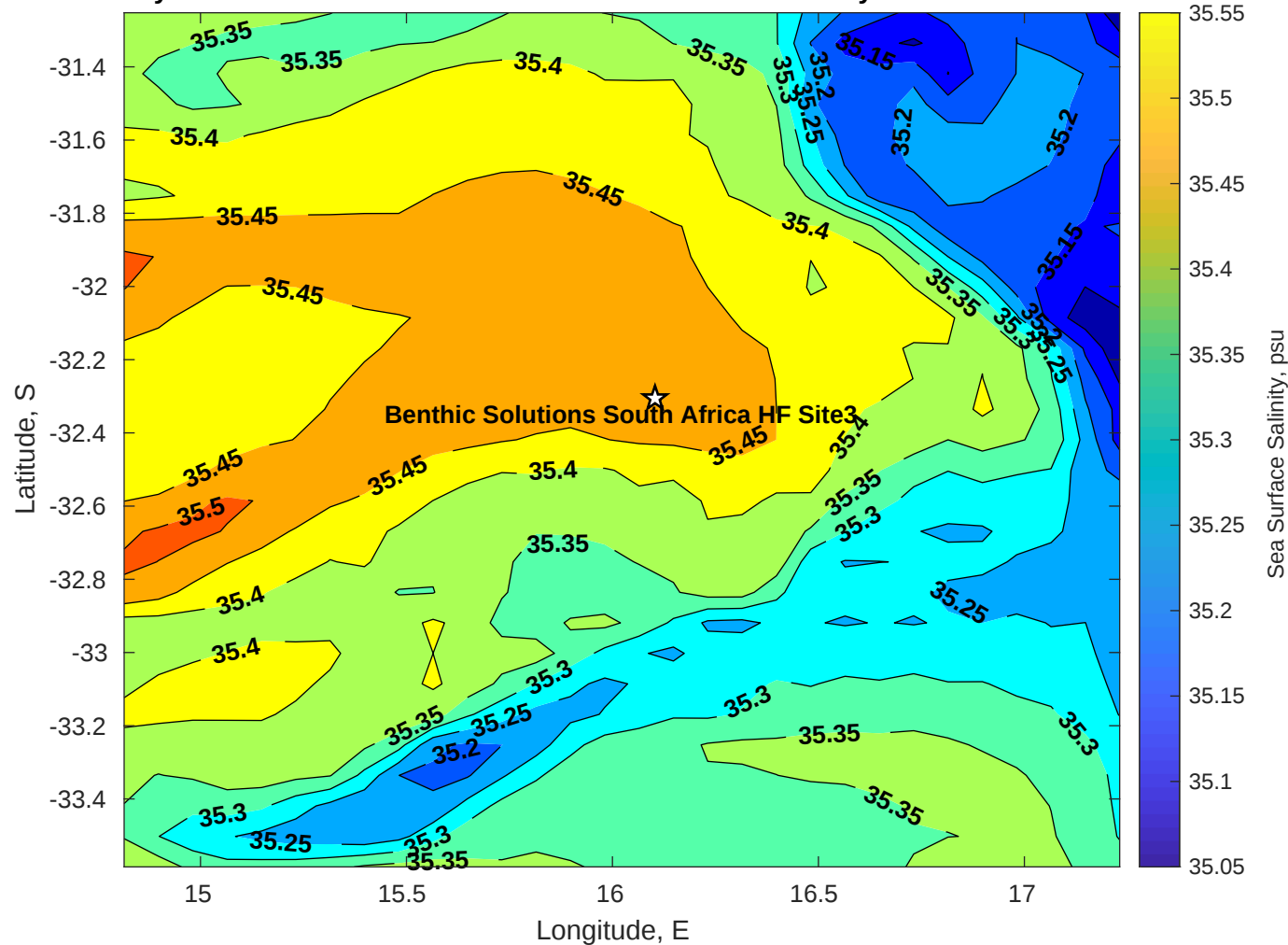
Surface Salinity for Benthic Solutions South Africa HF Site3 at 21-May-2025 00:00:00
