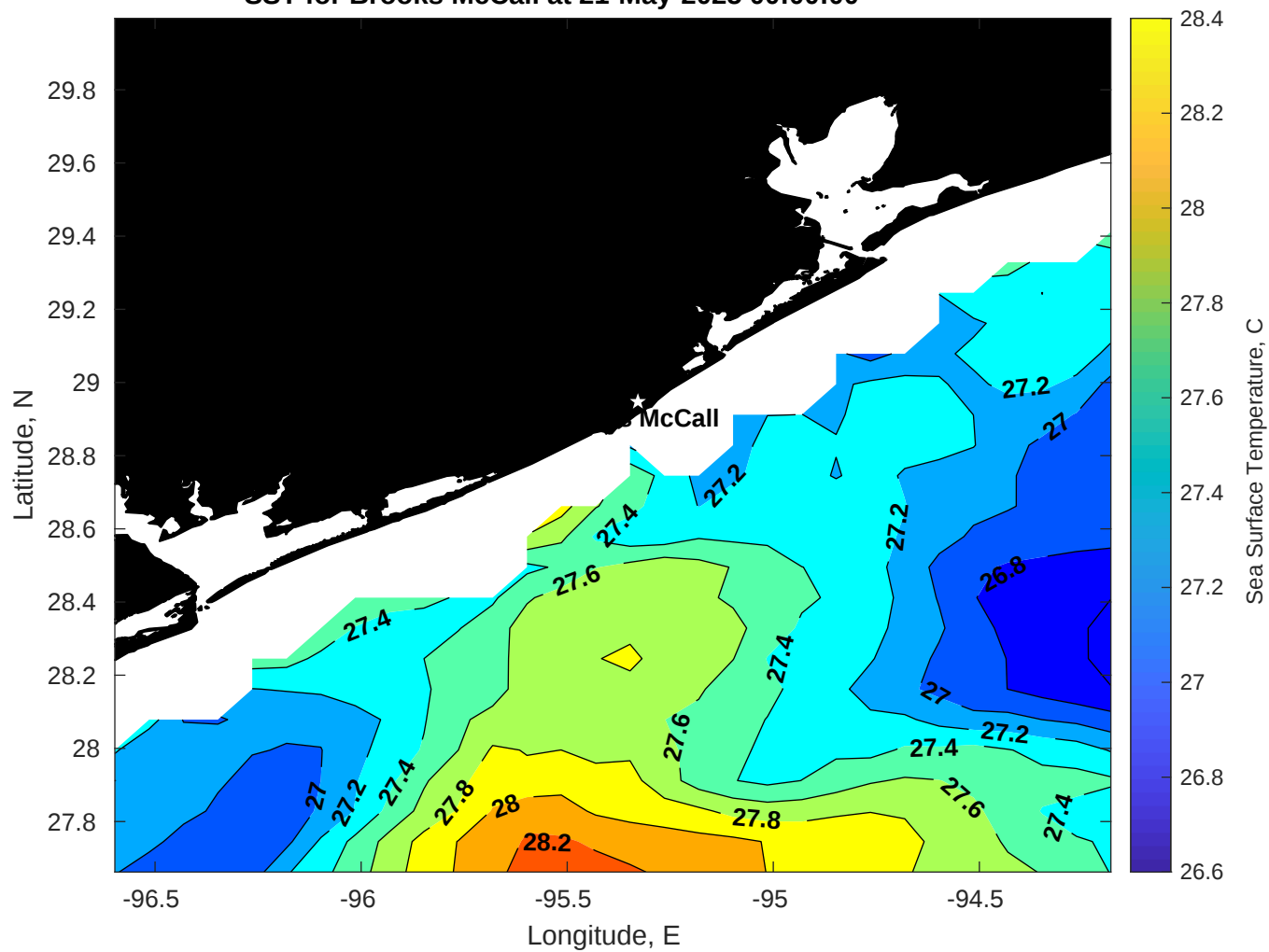
SST for Brooks McCall at 21-May-2025 00:00:00
