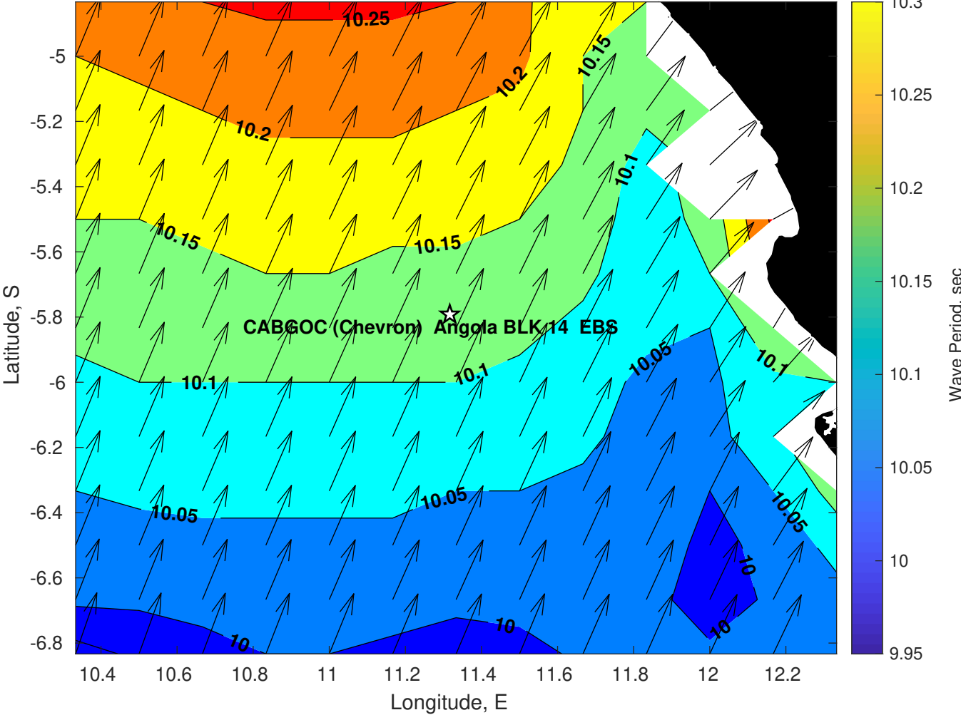
Wave Period (sec) for CABGOC (Chevron) Angola BLK 14 EBS at 22-May-2025 09:00:00
