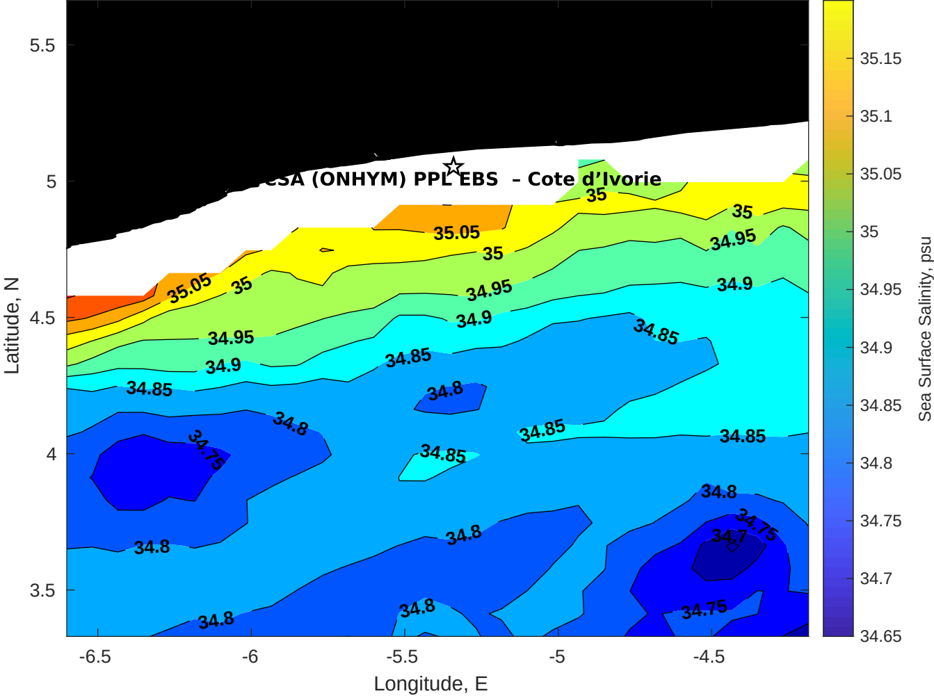
Surface Salinity for CSA (ONHYM) PPL EBS - Cote d'Ivoire at 21-May-2025 00:00:00
