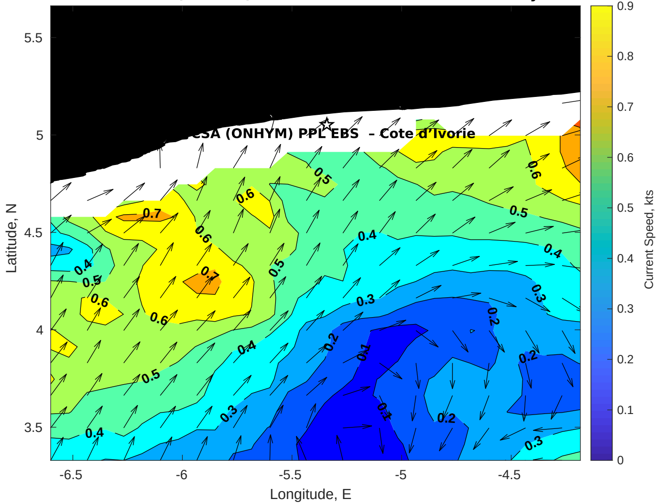
Surface Currents for CSA (ONHYM) PPL EBS - Cote d'Ivoire at 21-May-2025 00:00:00
