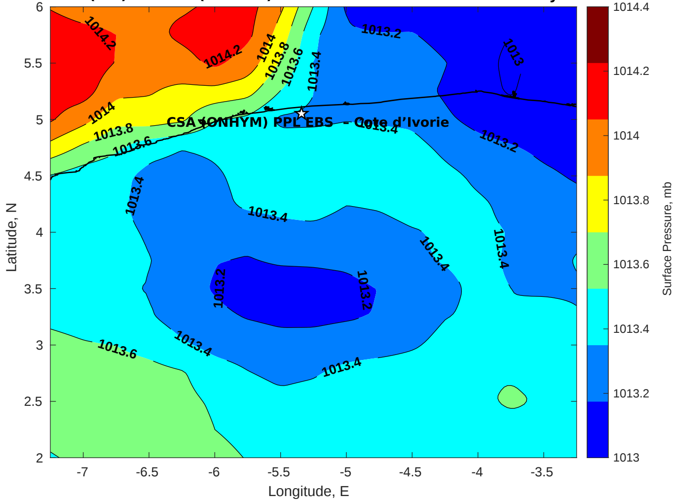
Surface Pressure (mb) for CSA (ONHYM) PPL EBS - Cote d'Ivoire at 24-May-2025 00:00:00
