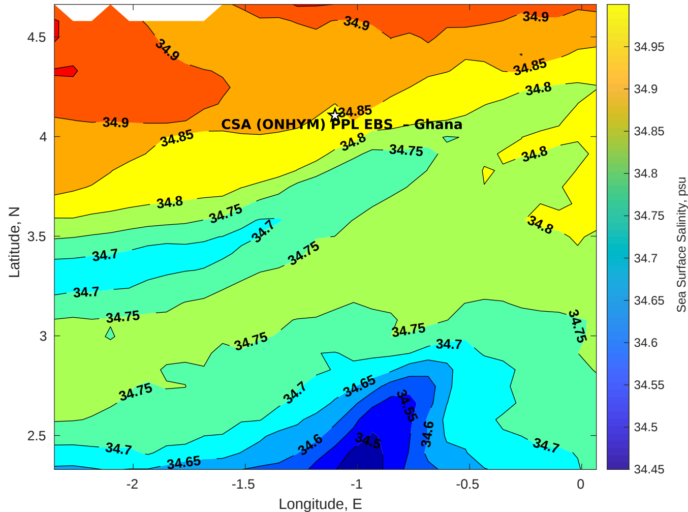
Surface Salinity for CSA (ONHYM) PPL EBS - Ghana at 21-May-2025 00:00:00
