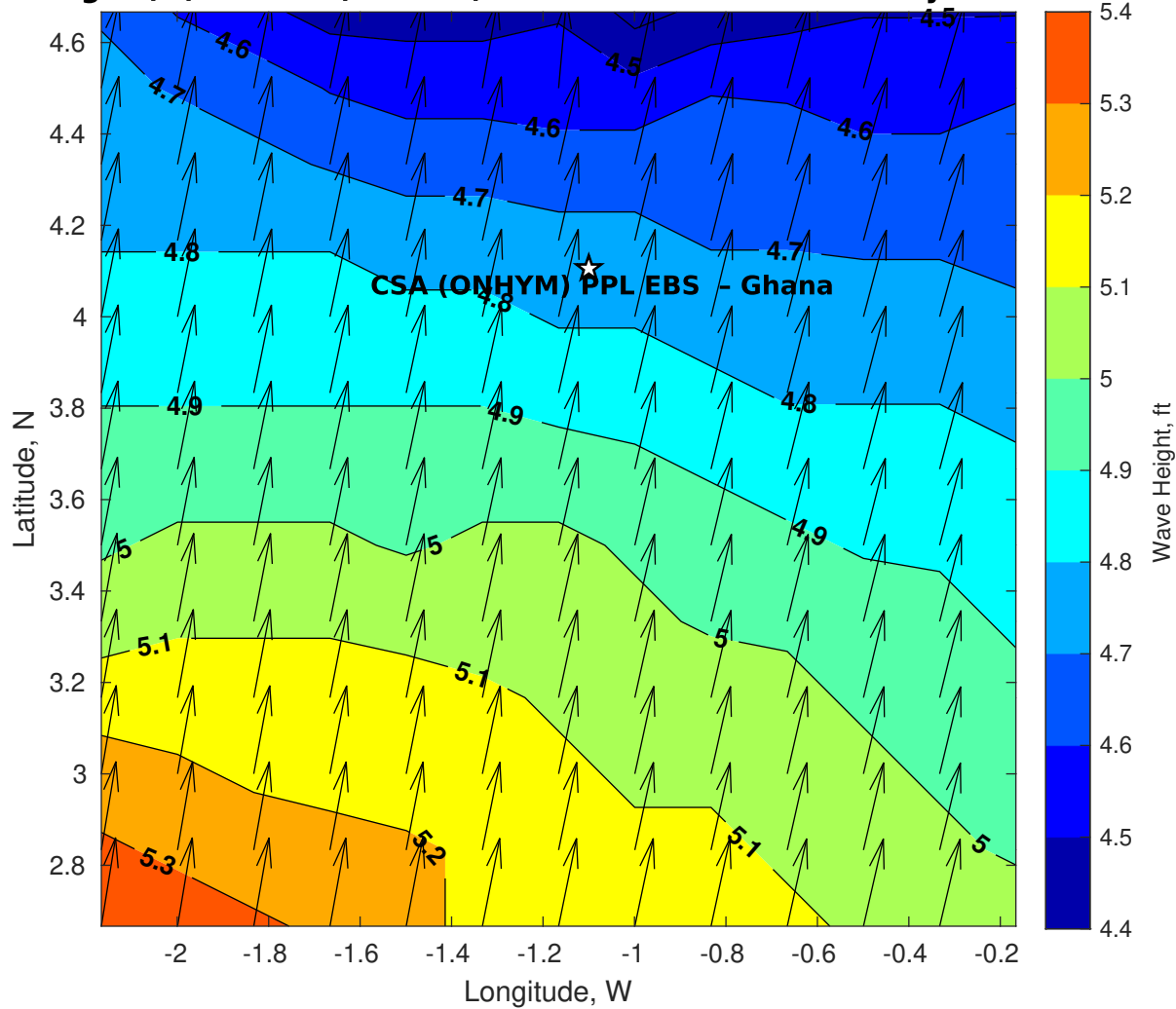
Wave Height (ft) for CSA (ONHYM) PPL EBS - Ghana at 22-May-2025 09:00:00
