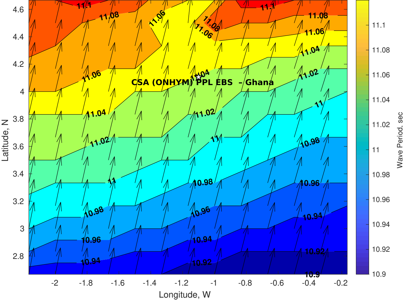
Wave Period (sec) for CSA (ONHYM) PPL EBS - Ghana at 22-May-2025 09:00:00
