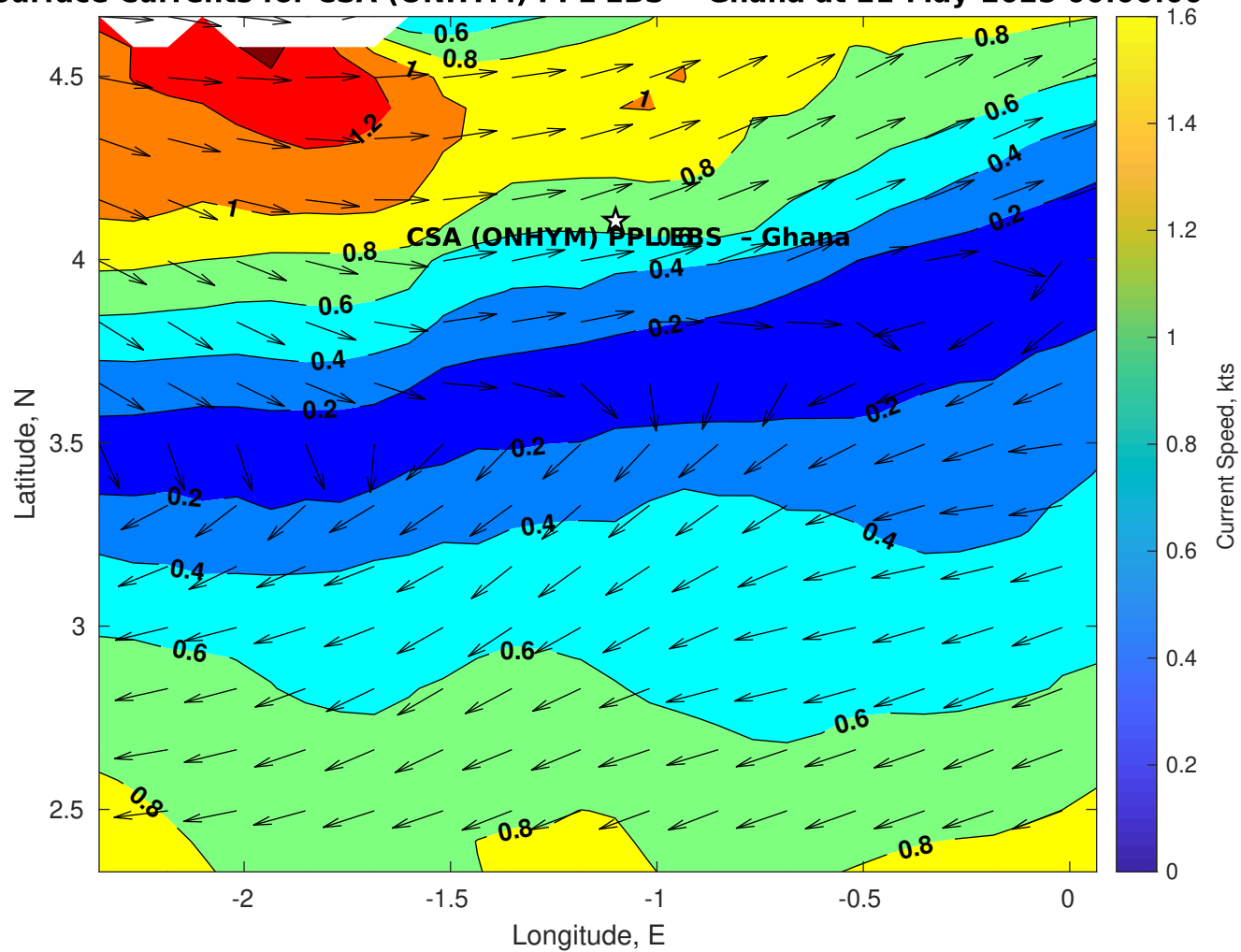
Surface Currents for CSA (ONHYM) PPL EBS - Ghana at 21-May-2025 00:00:00
