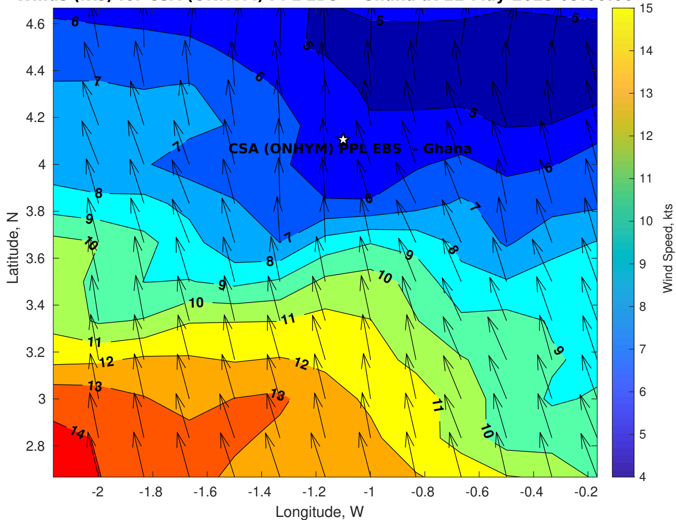
Winds (kts) for CSA (ONHYM) PPL EBS - Ghana at 22-May-2025 09:00:00
